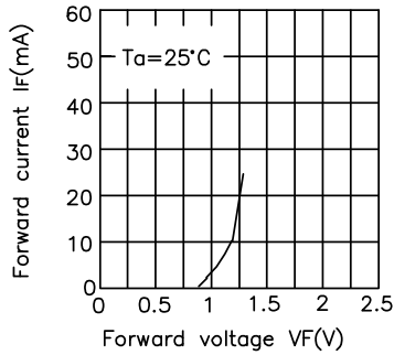
Fig.1 Forward Current vs. Forward Voltage(Typical)
