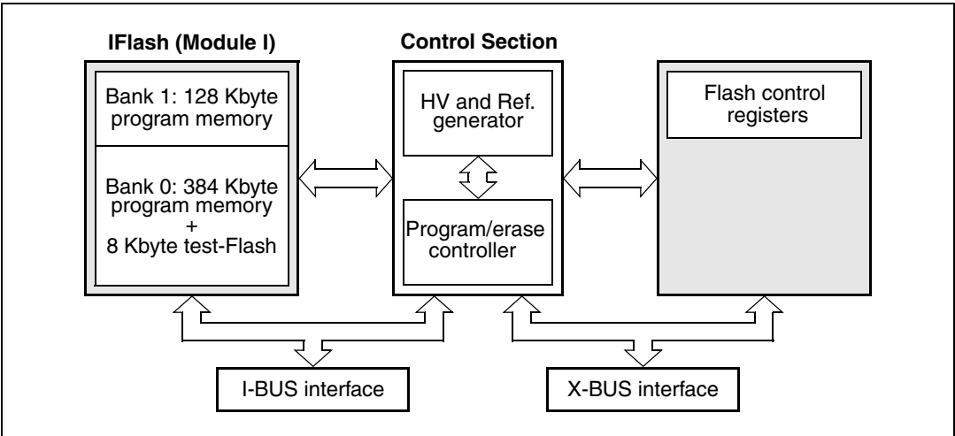
Figure 4. Flash structure
