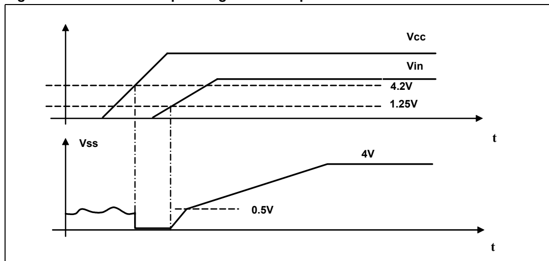
Figure 6. Device start-up: voltage at the SS pin
