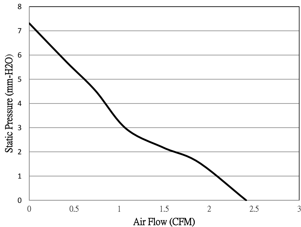
P-Q Curve
