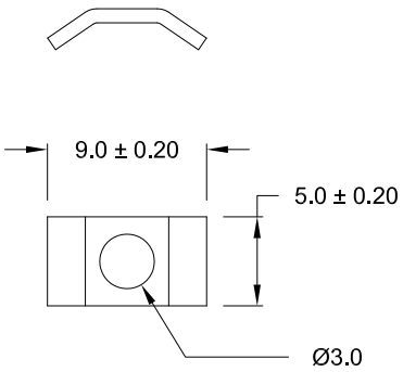
SADDLE WASHER
