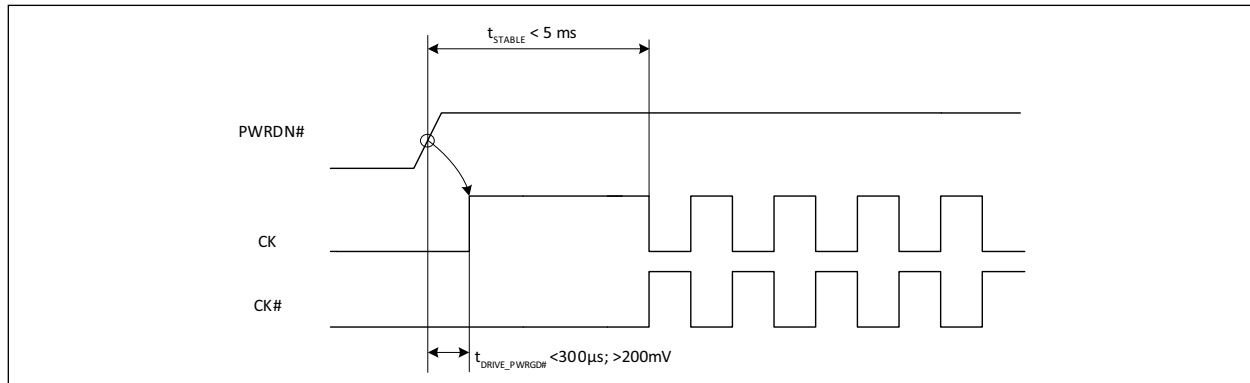
FIGURE 2-9: PWRGD Assertion.
