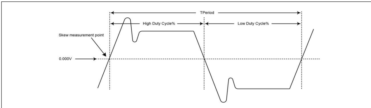
FIGURE 4-4: Differential Output Clock Measurement Points.
