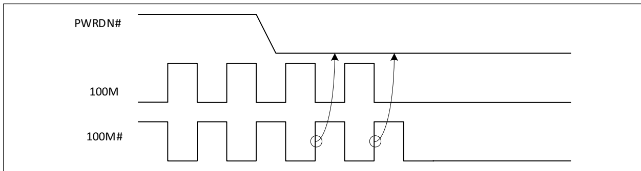
FIGURE 2-7: PWRDN# Assertion.
