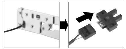
Crimp the connector on the cable. Quick connection to the sensor.
