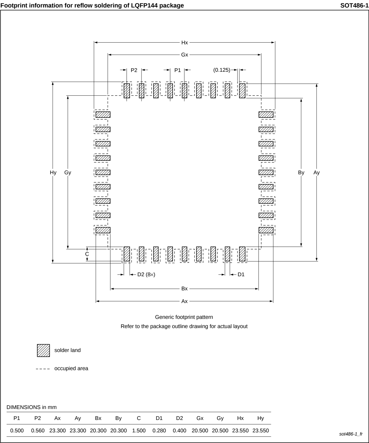
Fig 56. Reflow soldering of the LQFP144 package
