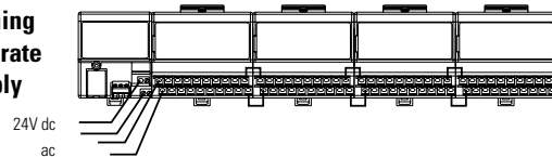
Wiring when total current draw is less than 10A
