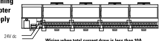
Wiring when total current draw is less than 10A
