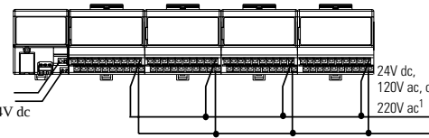
Wiring when total current draw is greater than 10A
