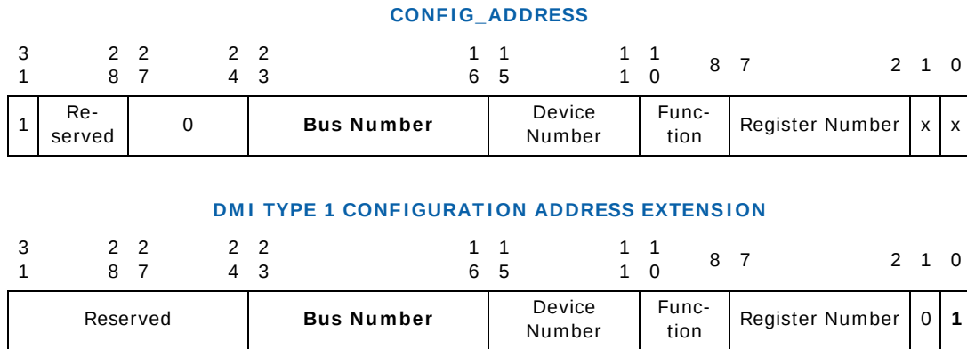
Figure 6. DMI Type 1 Configuration Address Translation
