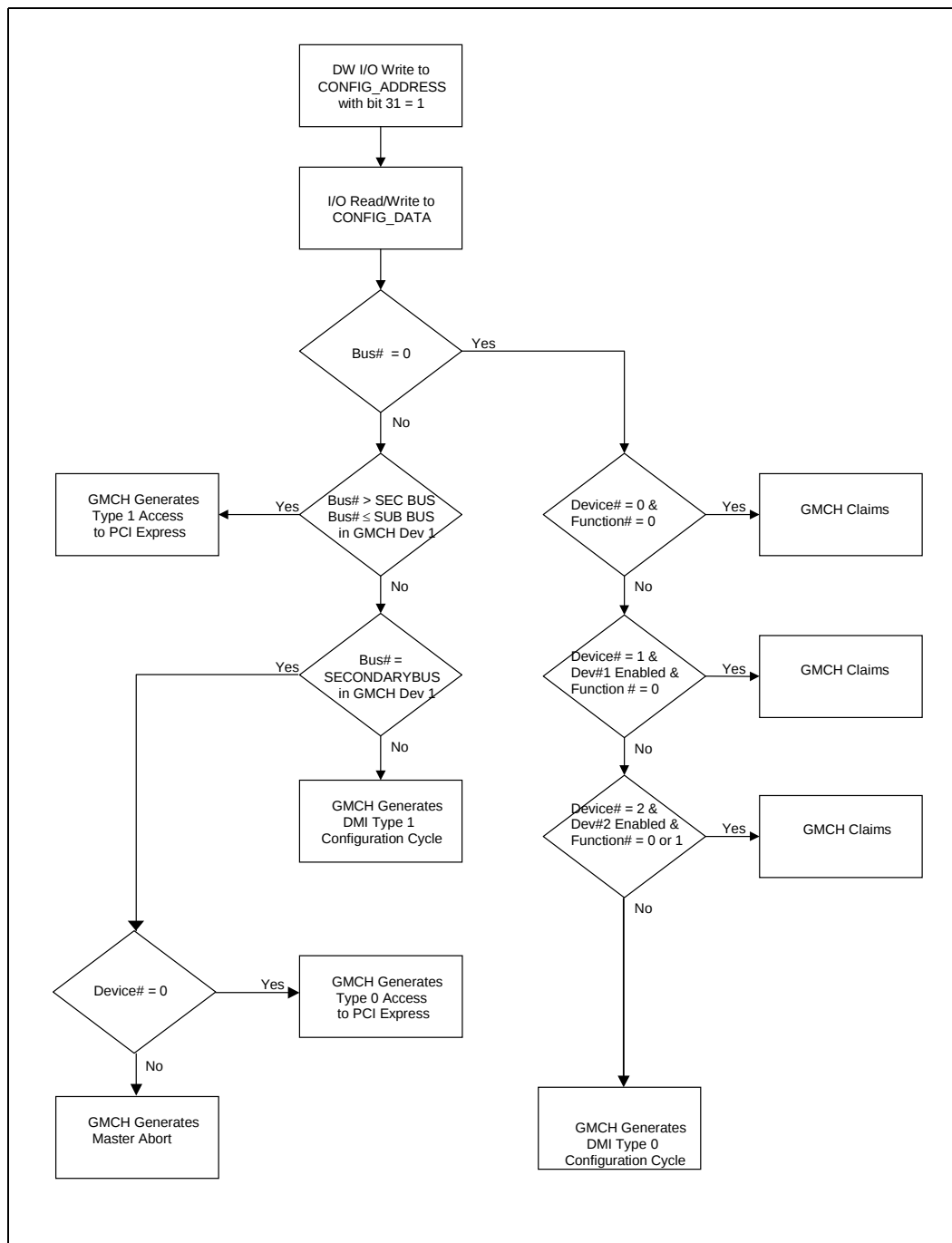
Figure 8. (G)MCH Configuration Cycle Flowchart
