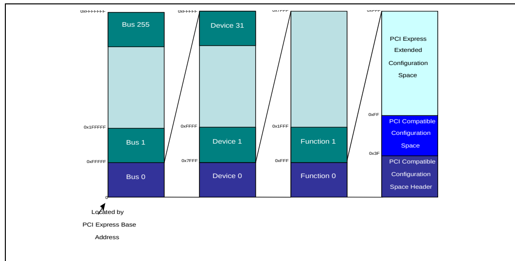
Figure 7. Memory Map to PCI Express Device Configuration Space
