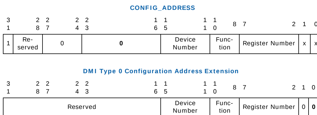
Figure 5. DMI Type 0 Configuration Address Translation
