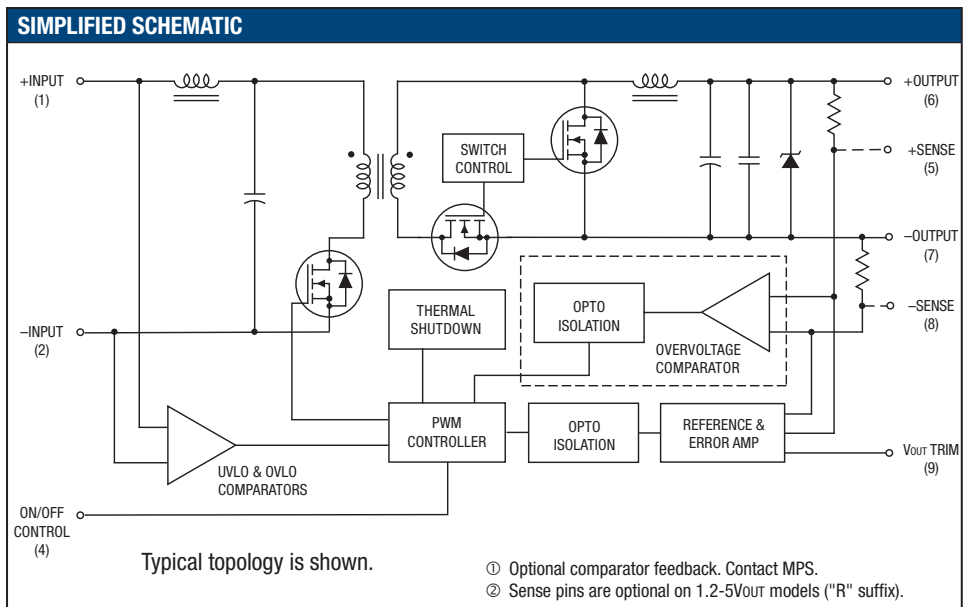
Figure 1. Simplified Schematic
