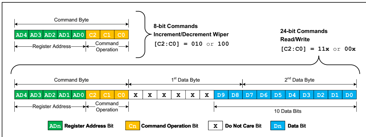
FIGURE 7-6: General SPI 8-Bit and 24-Bit Command Formats.
