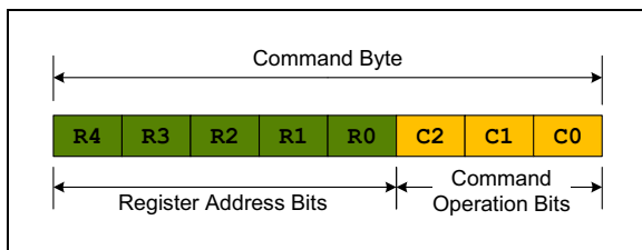
FIGURE 6-5: I 2 C Command Byte Format.
