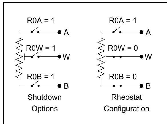
FIGURE 4-5: Resistor Network Terminal Configuration Options.
