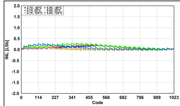
FIGURE 2-19: Rheostat Integral Nonlinearity (R-INL) Error vs. Wiper Position (Code), across V_{DD} and Temperature.
