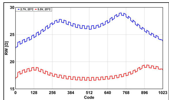
FIGURE 2-26: Wiper Resistance ( R_W ) in Rheostat Mode vs. Wiper Position (Code), across V_{DD} and Temperature.
