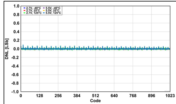
FIGURE 2-20: Rheostat Differential Nonlinearity (R-DNL) Error vs. Wiper Position (Code), across V_{DD} and Temperature.
