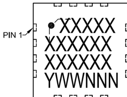
16-Lead VQFN, 4x4 mm Body
