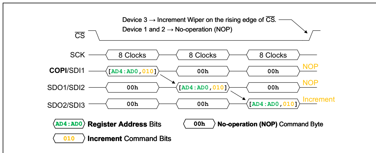
FIGURE 7-14: SPI Daisy-Chain Addressable 8-Bit Increment/Decrement Commands Example.
