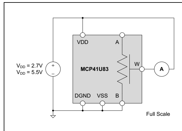
FIGURE B-4: Test Circuit for R_{WB} and R-R_{TC} .
