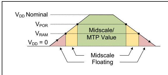
FIGURE 4-3: Power-up and Power-down.
