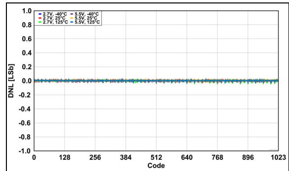
FIGURE 2-25: Rheostat Differential Nonlinearity (R-DNL) Error vs. Wiper Position (Code), across V_{DD} and Temperature.
