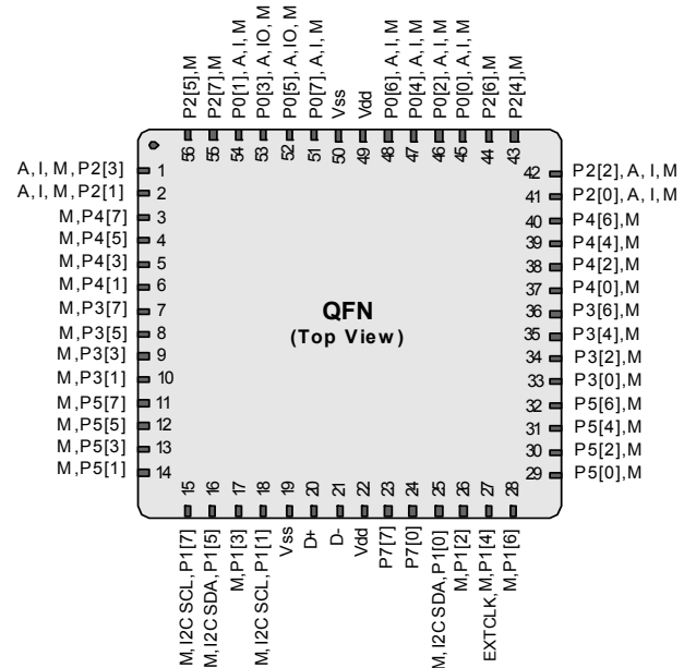
Figure 4. CY8C24794 56-Pin PSoC Device [3]
