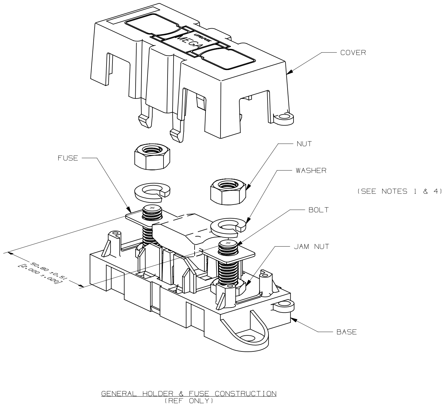
GENERAL HOLDER & FUSE CONSTRUCTION (REF ONLY)
