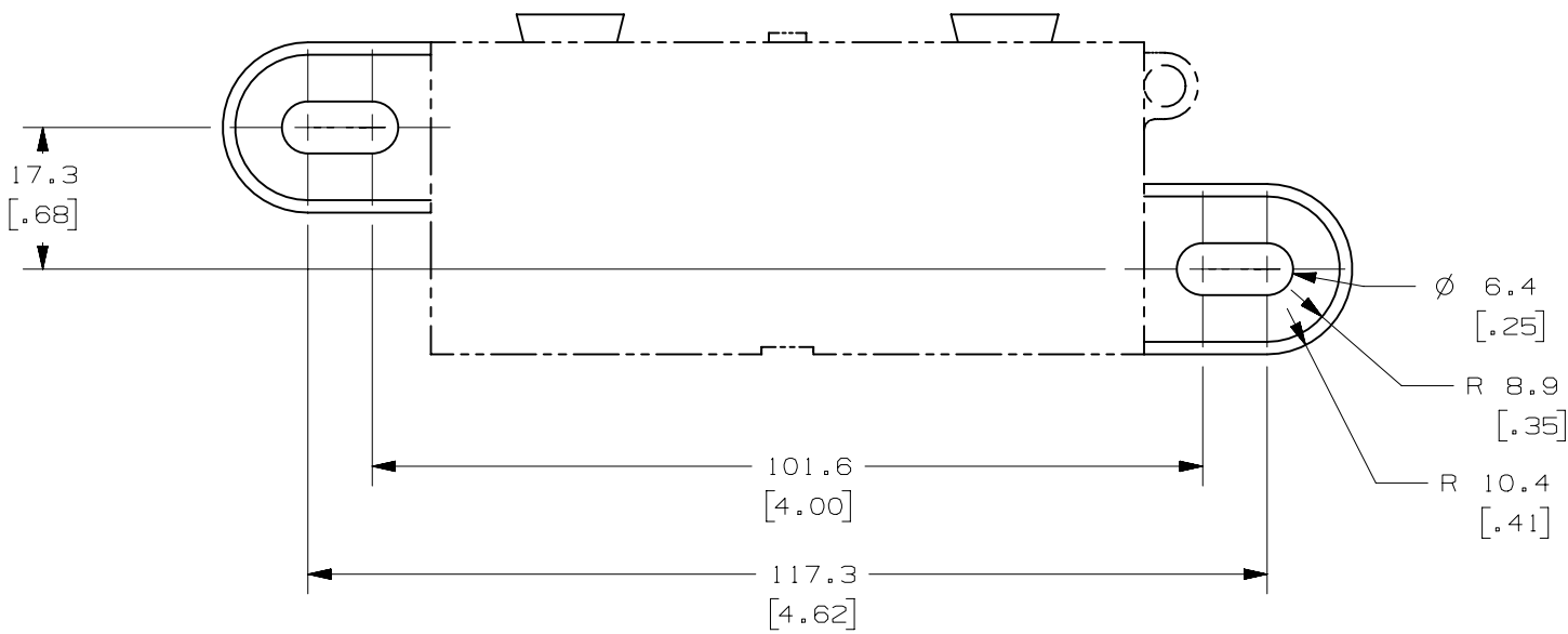
VERSION WITH EXTENDED MOUNTING CENTERS BASE STYLE 2
