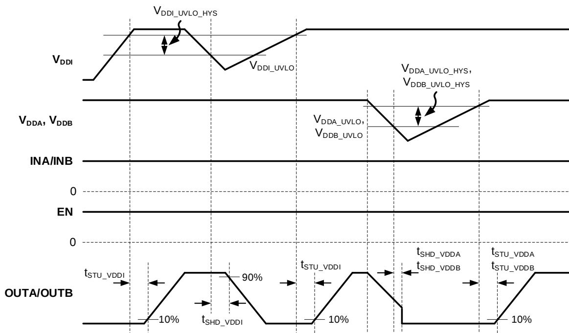
Figure 4: V DDI and V DDA , V DDB Under-Voltage Lockout (UVLO)
