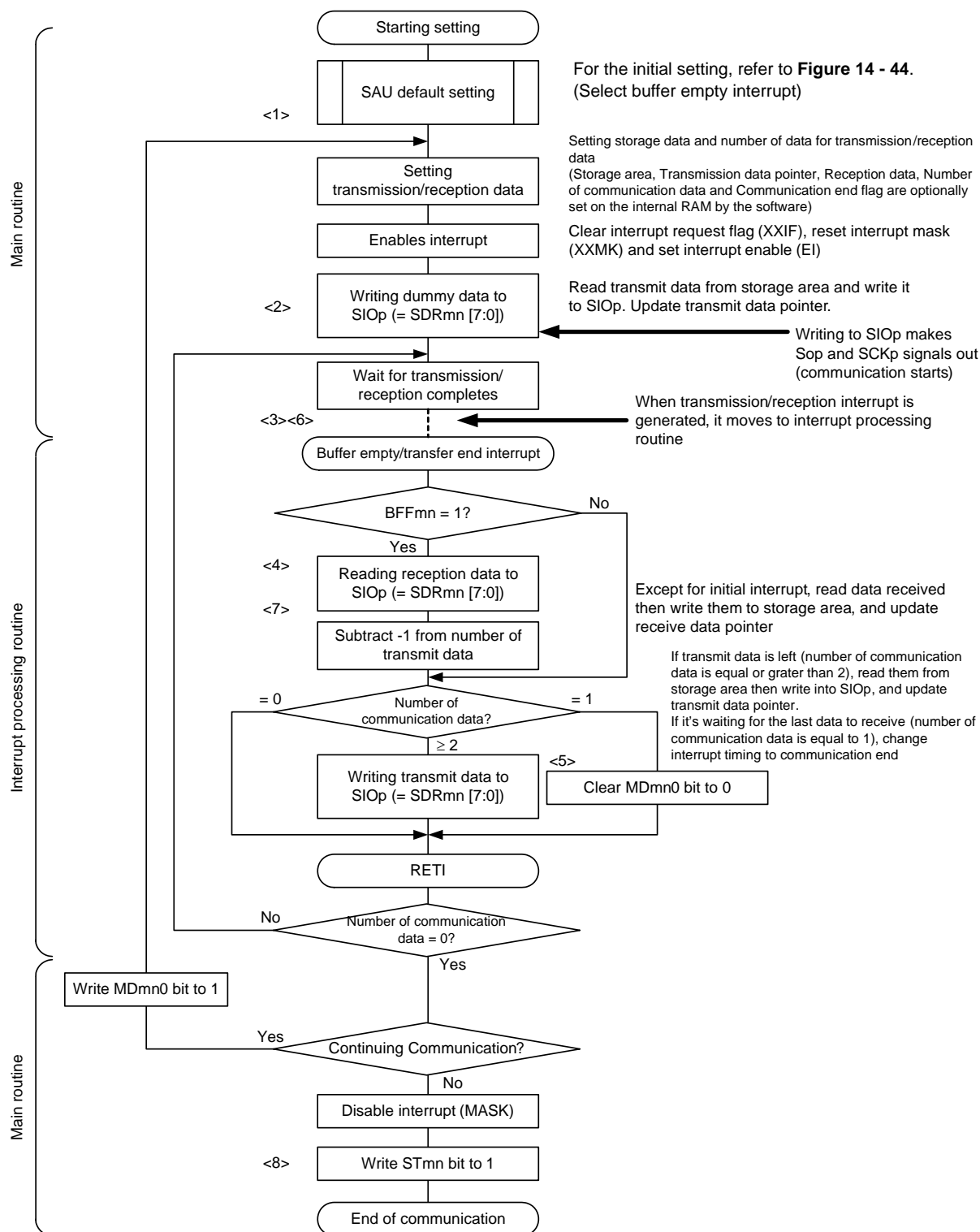
&lt;R&gt; Figure 14 - 50 Flowchart of Master Transmission/Reception (in Continuous Transmission/Reception Mode)
