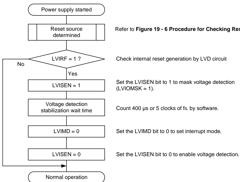
Figure 21 - 9 Setting Procedure for Initial Setting of Interrupt and Reset Mode
