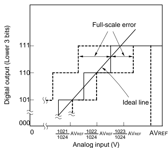
Figure 12 - 43 Full-Scale Error
