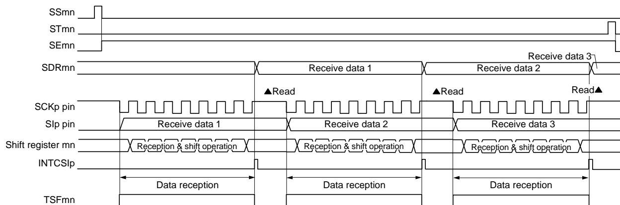
<R> Figure 14 - 63 Timing Chart of Slave Reception (in Single-Reception Mode) (Type 1: DAPmn = 0, CKPmn = 0)
