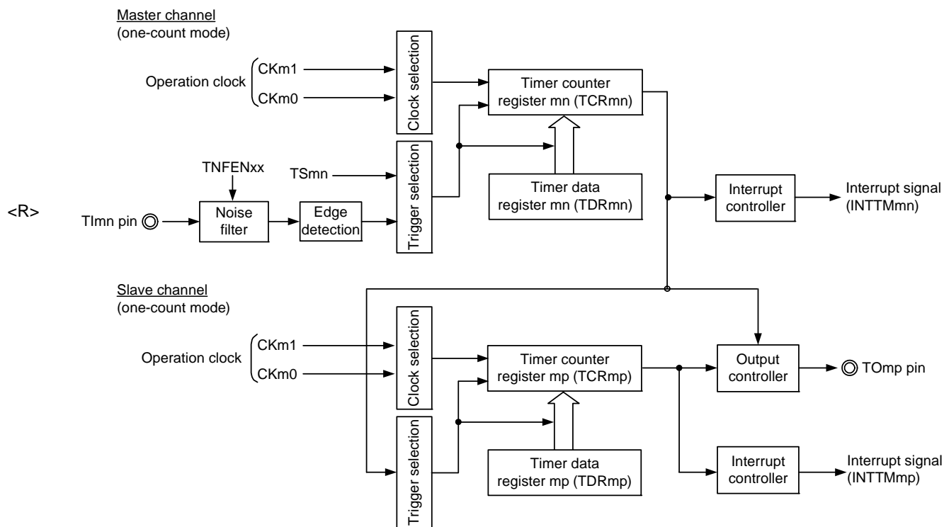
Figure 6 - 70 Block Diagram of Operation as One-Shot Pulse Output Function
