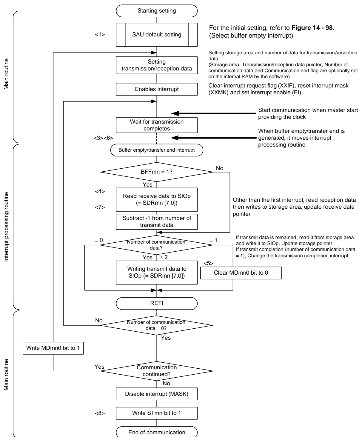
<R> Figure 14 - 104 Flowchart of Slave Transmission/Reception (in Continuous Transmission/Reception Mode)
