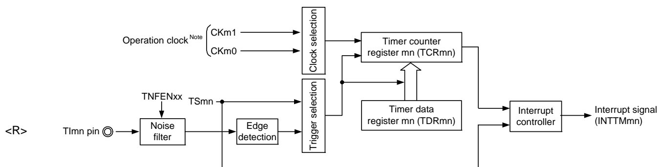
Figure 6 - 66 Block Diagram of Operation as Delay Counter
