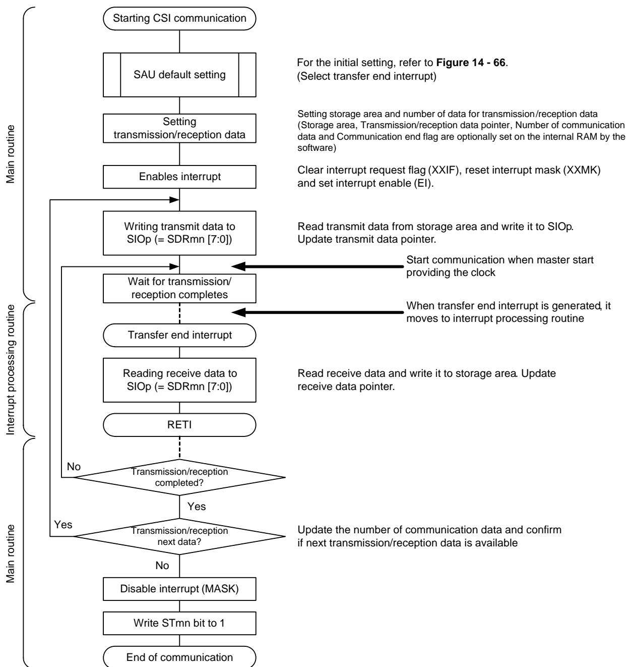
<R> Figure 14 - 70 Flowchart of Slave Transmission/Reception (in Single-Transmission/Reception Mode)
