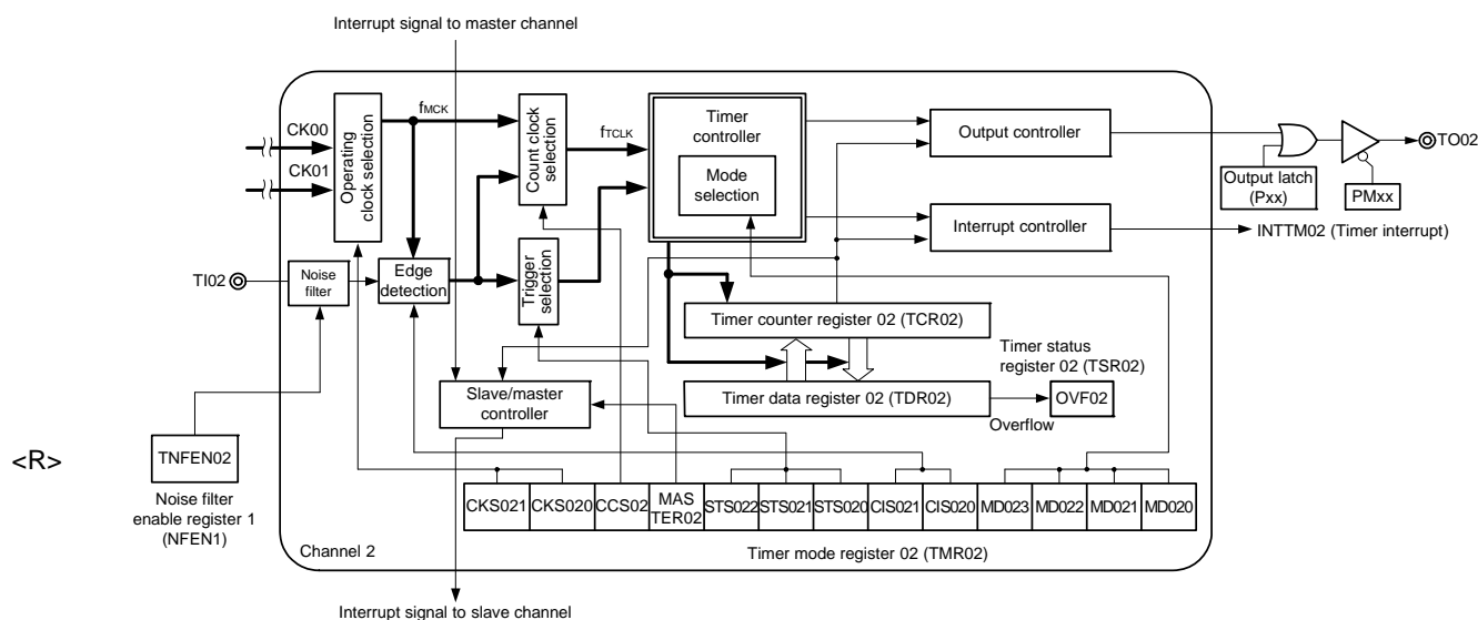
Figure 6 - 4 Internal Block Diagram of Channel 2 of Timer Array Unit 0
