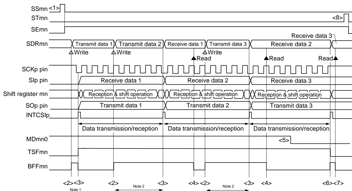
<R> Figure 14 - 71 Timing Chart of Slave Transmission/Reception (in Continuous Transmission/Reception Mode) (Type 1: DAPmn = 0, CKPmn = 0)
