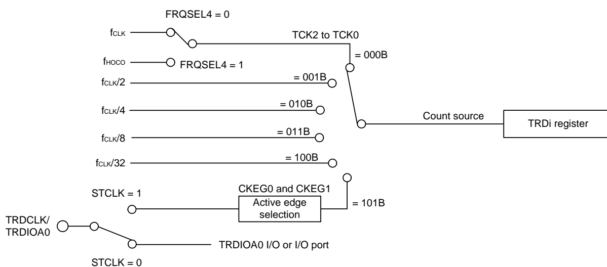
Figure 8 - 41 Count Source Block Diagram
