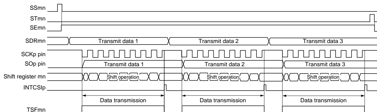
Figure 14 - 55 Timing Chart of Slave Transmission (in Single-Transmission Mode)
