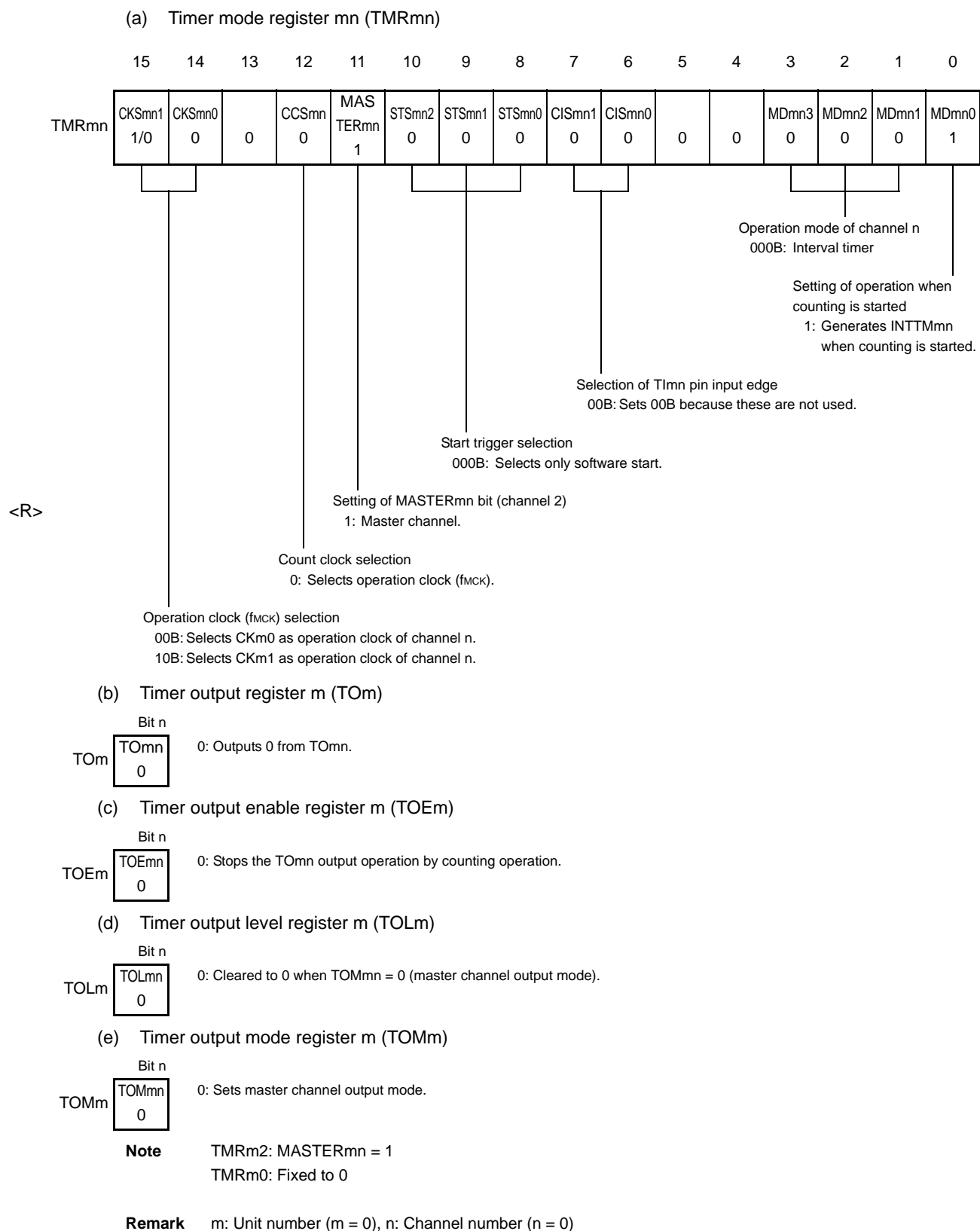
Figure 6 - 84 Example of Set Contents of Registers When Multiple PWM Output Function (Master Channel) Is Used
