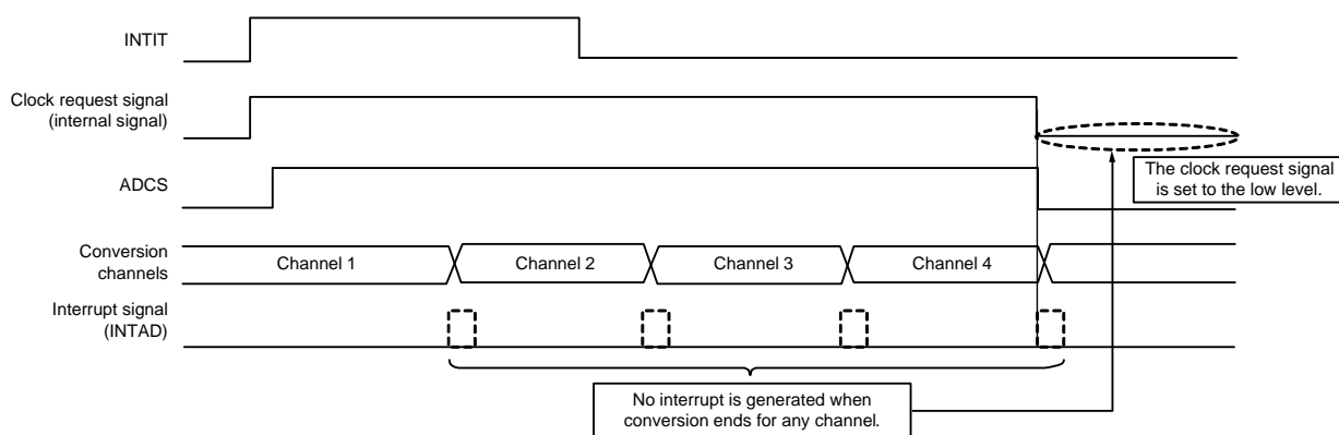
Figure 12 - 38 Operation Example When No Interrupt Is Generated After A/D Conversion Ends (While in Scan Mode)
