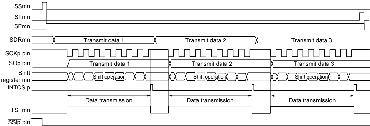
<R> Figure 14 - 85 Timing Chart of Slave Transmission (in Single-Transmission Mode) (Type 1: DAPmn = 0, CKPmn = 0)
