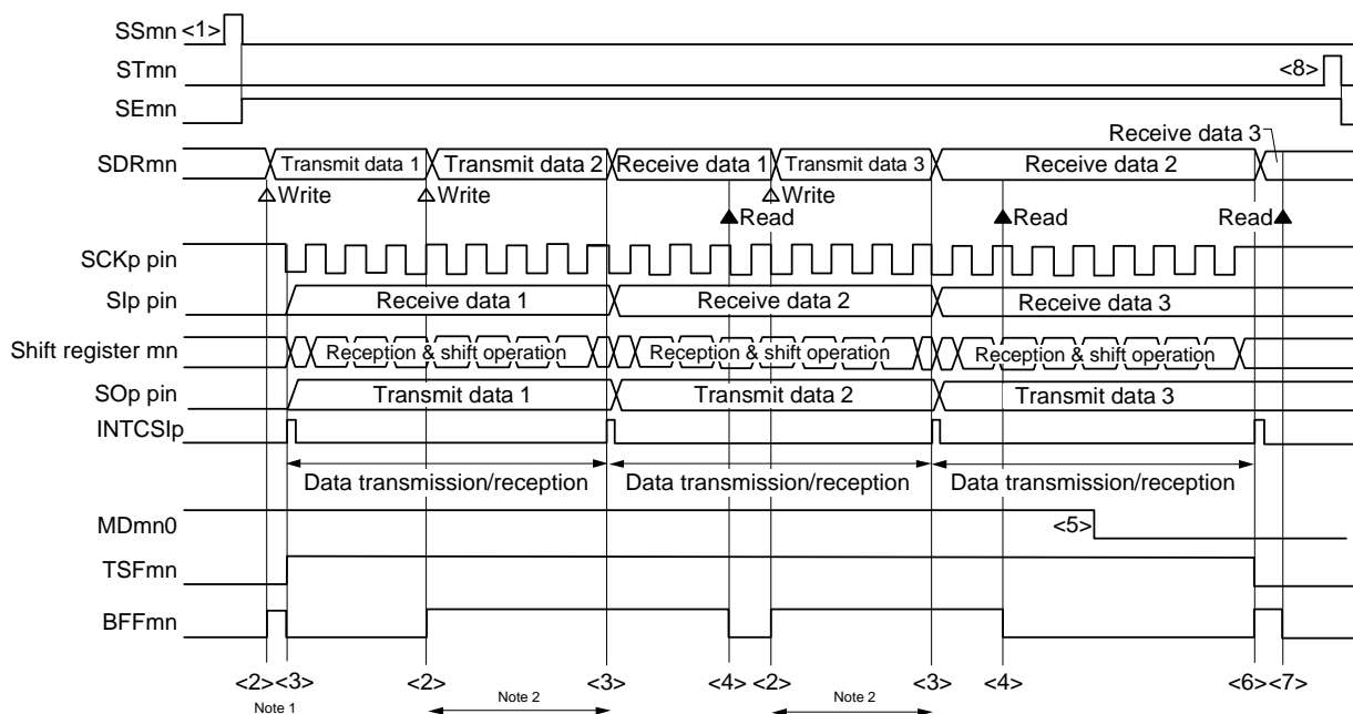
<R> Figure 14 - 49 Timing Chart of Master Transmission/Reception (in Continuous Transmission/Reception Mode) (Type 1: DAPmn = 0, CKPmn = 0)
