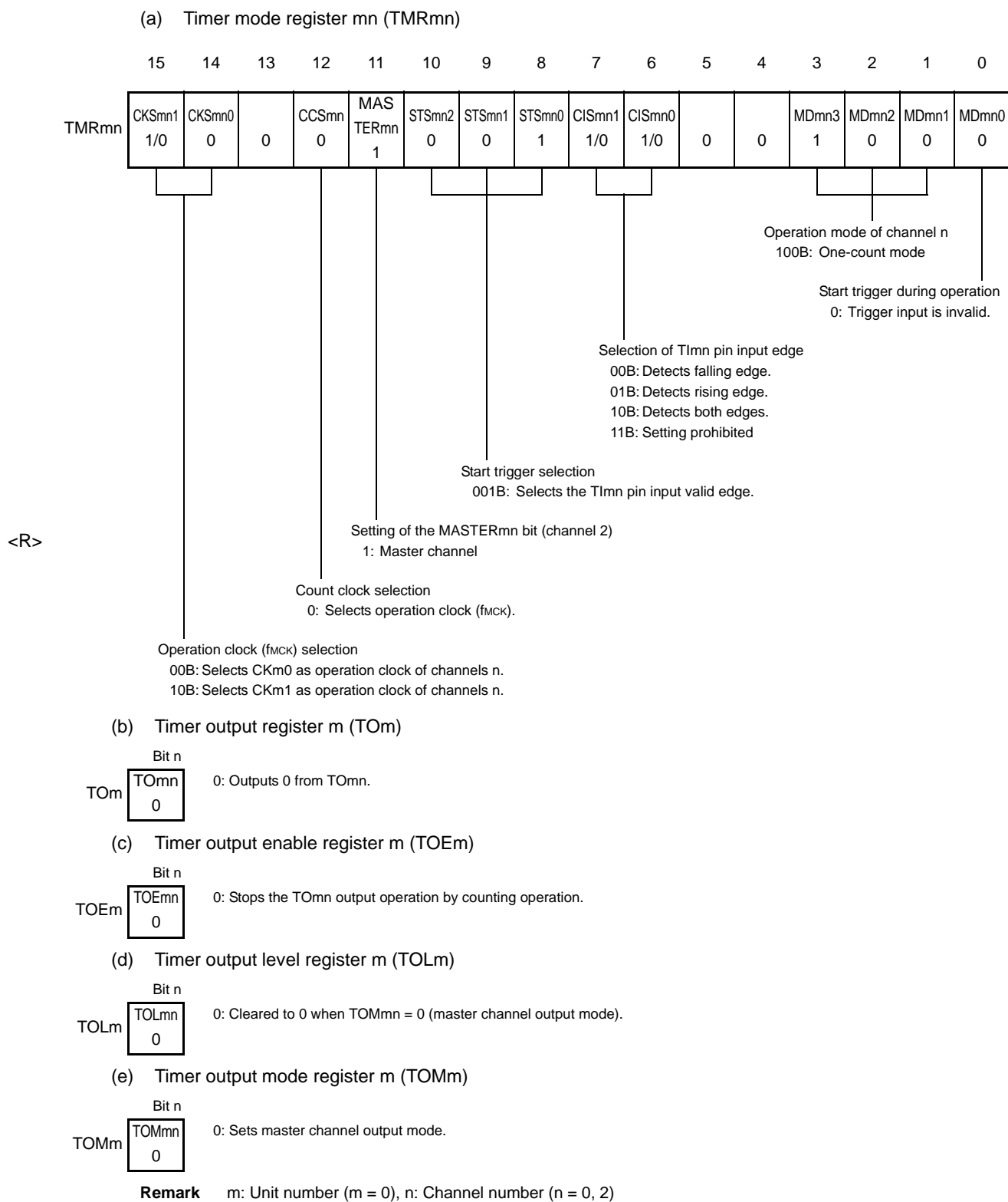
Figure 6 - 72 Example of Set Contents of Registers When One-Shot Pulse Output Function Is Used (Master Channel)
