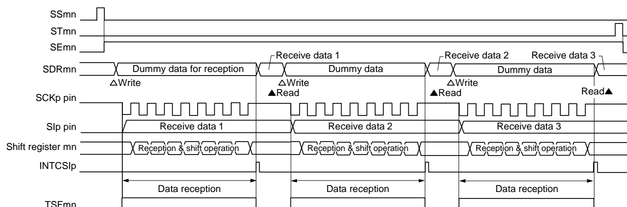
<R> Figure 14 - 39 Timing Chart of Master Reception (in Single-Reception Mode) (Type 1: DAPmn = 0, CKPmn = 0)
