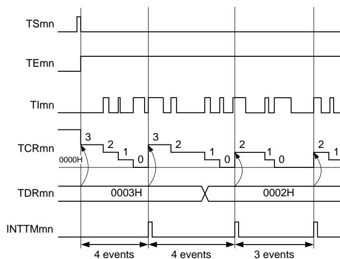
Figure 6 - 51 Example of Basic Timing of Operation as External Event Counter
