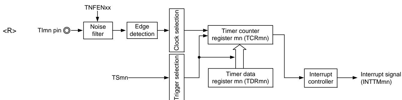
Figure 6 - 50 Block Diagram of Operation as External Event Counter
