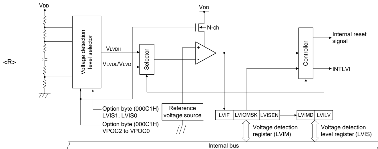
Figure 21 - 1 Block Diagram of Voltage Detector
