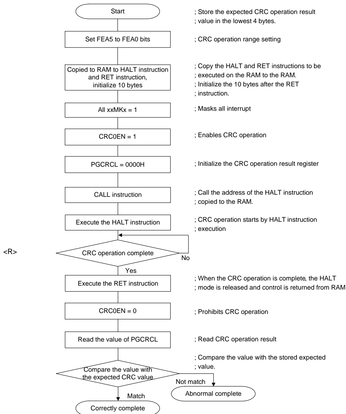
Figure 22 - 3 Flowchart of Flash Memory CRC Operation Function (High-speed CRC)
