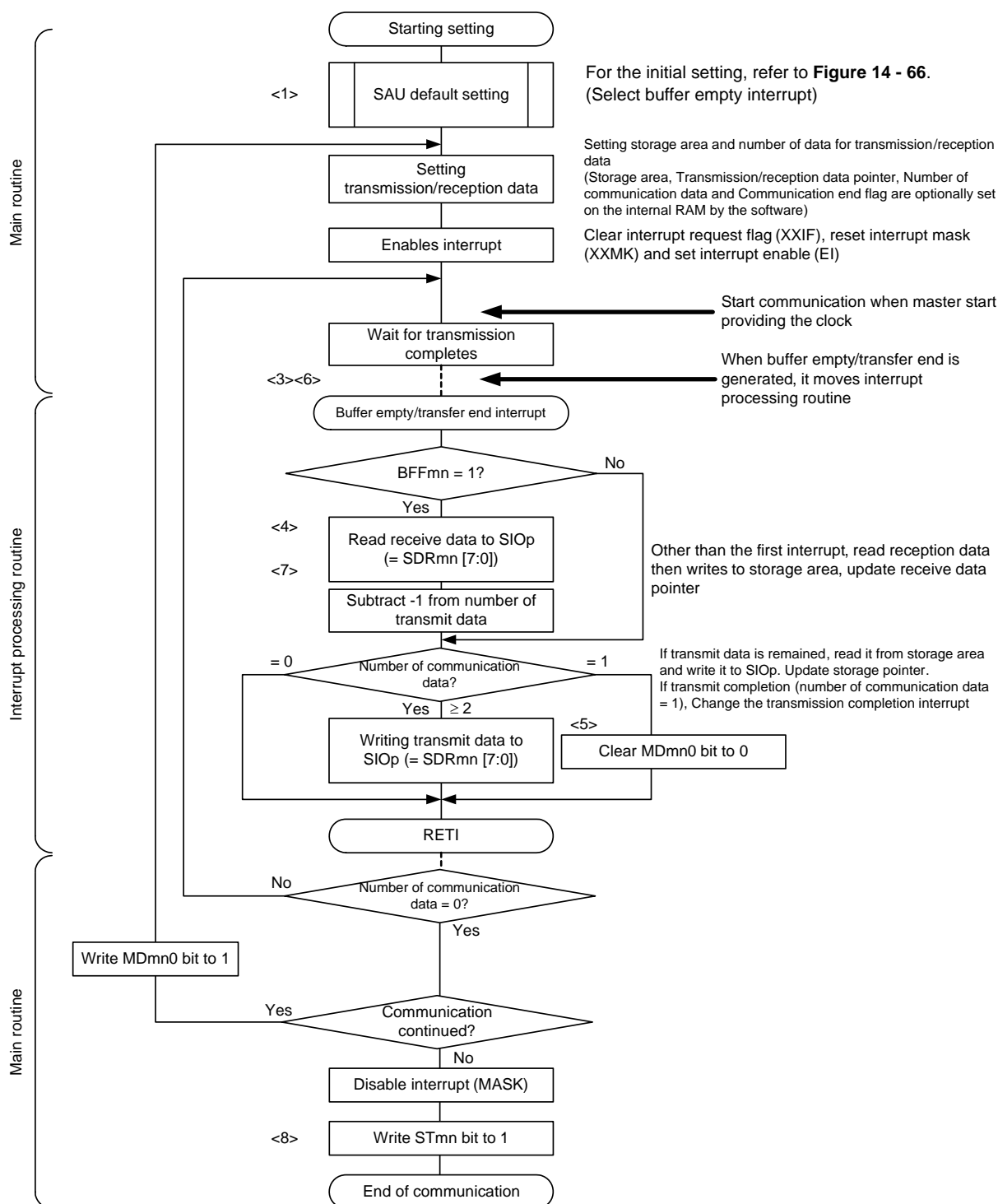
&lt;R&gt; Figure 14 - 72 Flowchart of Slave Transmission/Reception (in Continuous Transmission/Reception Mode)
