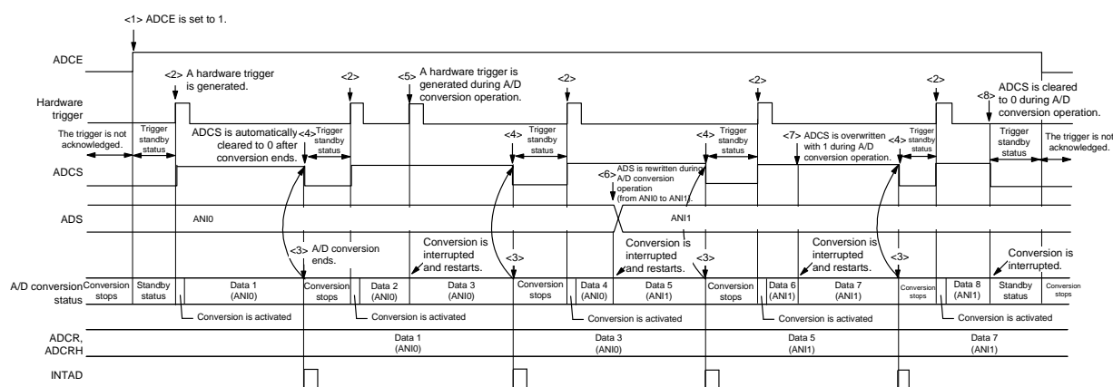
Figure 12 - 28 Example of Hardware Trigger Wait Mode (Select Mode, One-Shot Conversion Mode) Operation
