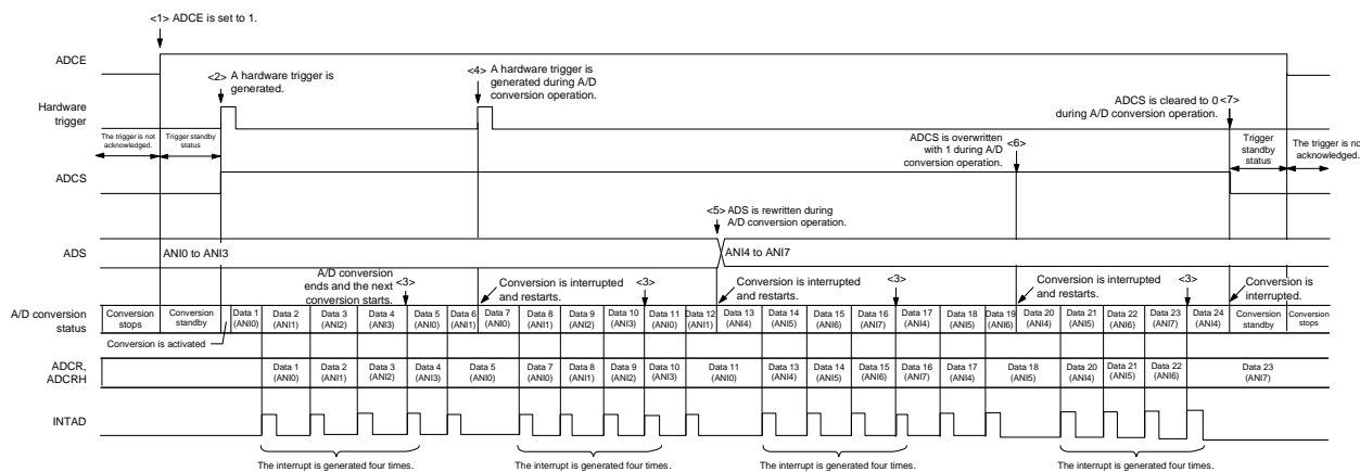
<R> Figure 12 - 29 Example of Hardware Trigger Wait Mode (Scan Mode, Sequential Conversion Mode) Operation Timing
