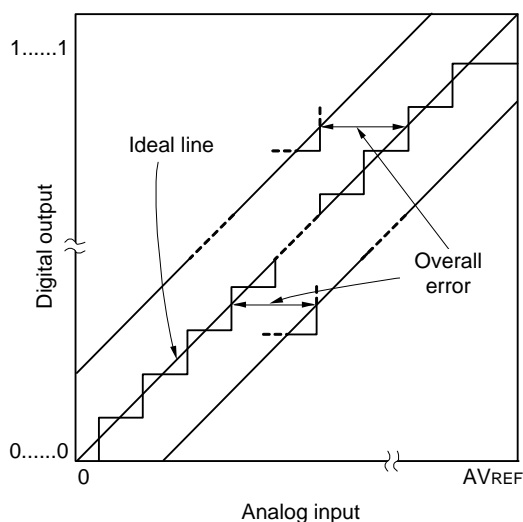
Figure 12 - 40 Overall Error
