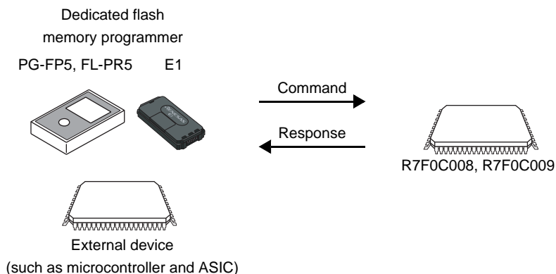
Figure 25 - 8 Communication Commands
