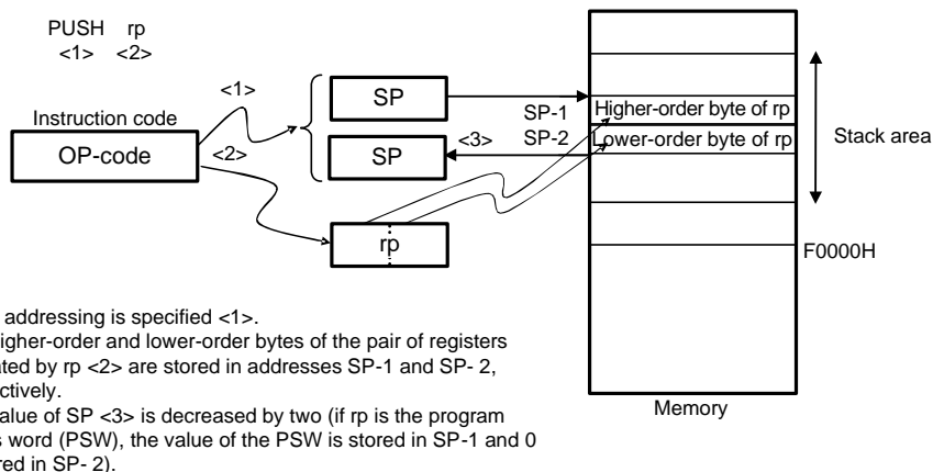
Figure 3 - 35 Example of PUSH rp
