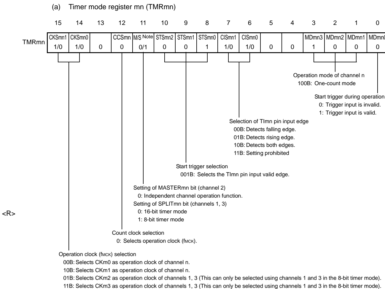
Figure 6 - 68 Example of Set Contents of Registers to Delay Counter
