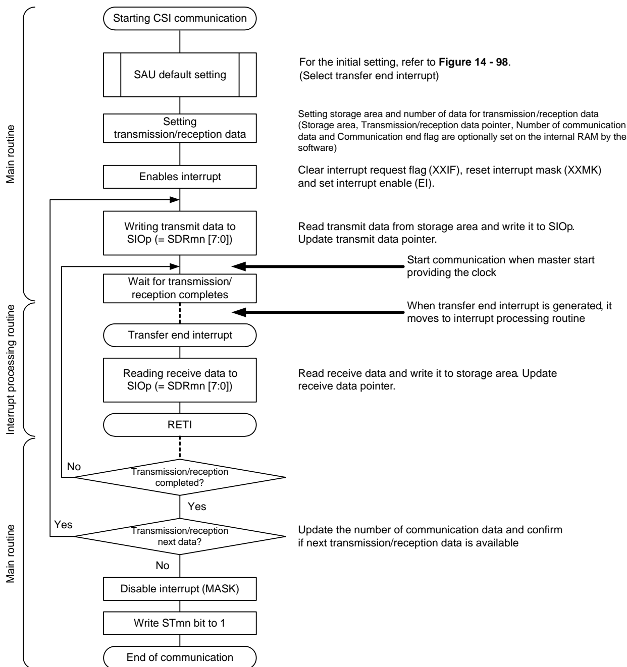
<R> Figure 14 - 102 Flowchart of Slave Transmission/Reception (in Single-Transmission/Reception Mode)
