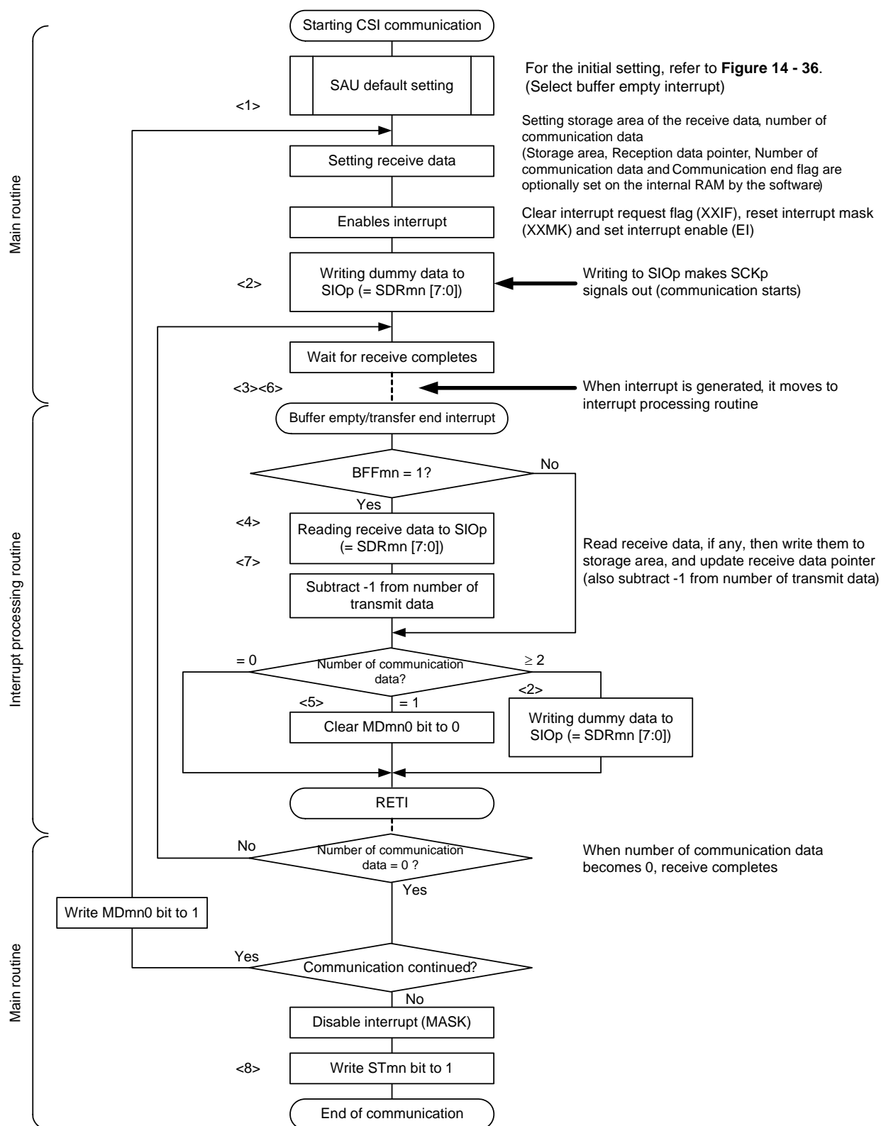
<R> Figure 14 - 42 Flowchart of Master Reception (in Continuous Reception Mode)
