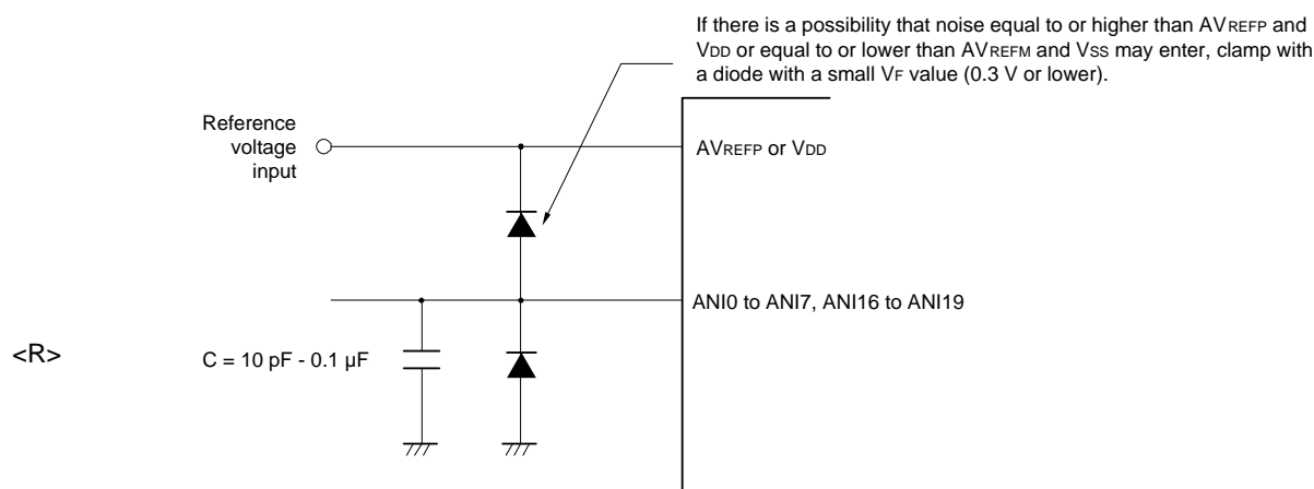
Figure 12 - 46 Analog Input Pin Connection
