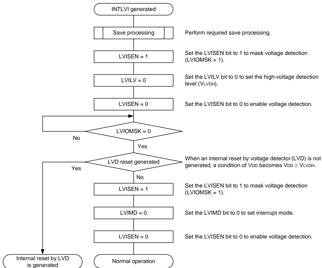
<R> Figure 21 - 8 Setting Procedure for Operating Voltage Check and Reset
