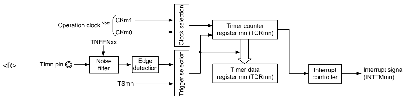
Figure 6 - 58 Block Diagram of Operation as Input Pulse Interval Measurement
