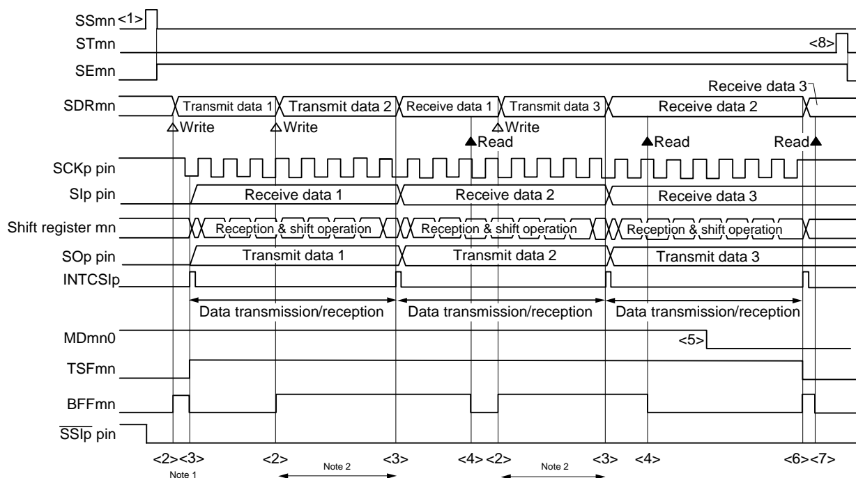
<R> Figure 14 - 103 Timing Chart of Slave Transmission/Reception (in Continuous Transmission/Reception Mode) (Type 1: DAPmn = 0, CKPmn = 0)
