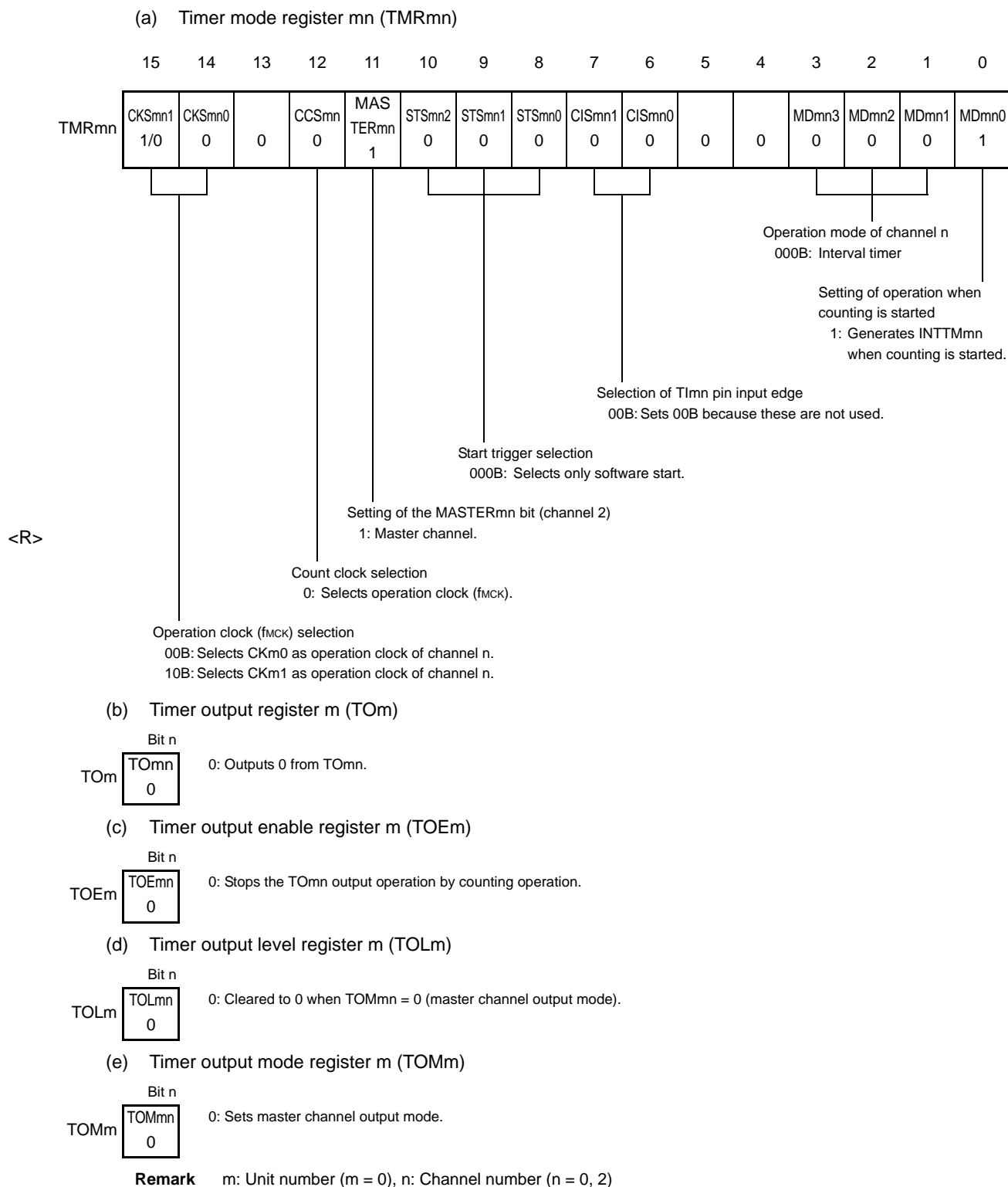
Figure 6 - 78 Example of Set Contents of Registers When PWM Function (Master Channel) Is Used
