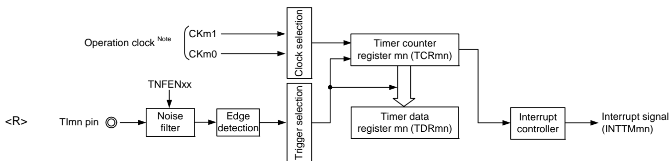
Figure 6 - 62 Block Diagram of Operation as Input Signal High-/Low-level Width Measurement
