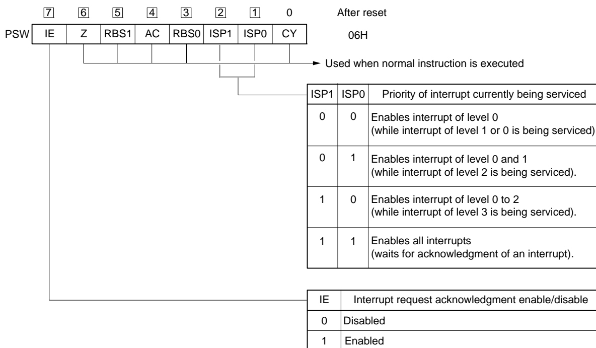
Figure 16 - 10 Configuration of Program Status Word
