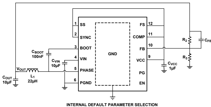
FIGURE 1. TYPICAL APPLICATION
