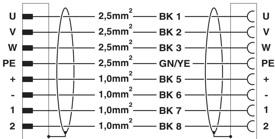
Contact assignment of M40 plugs/sockets
