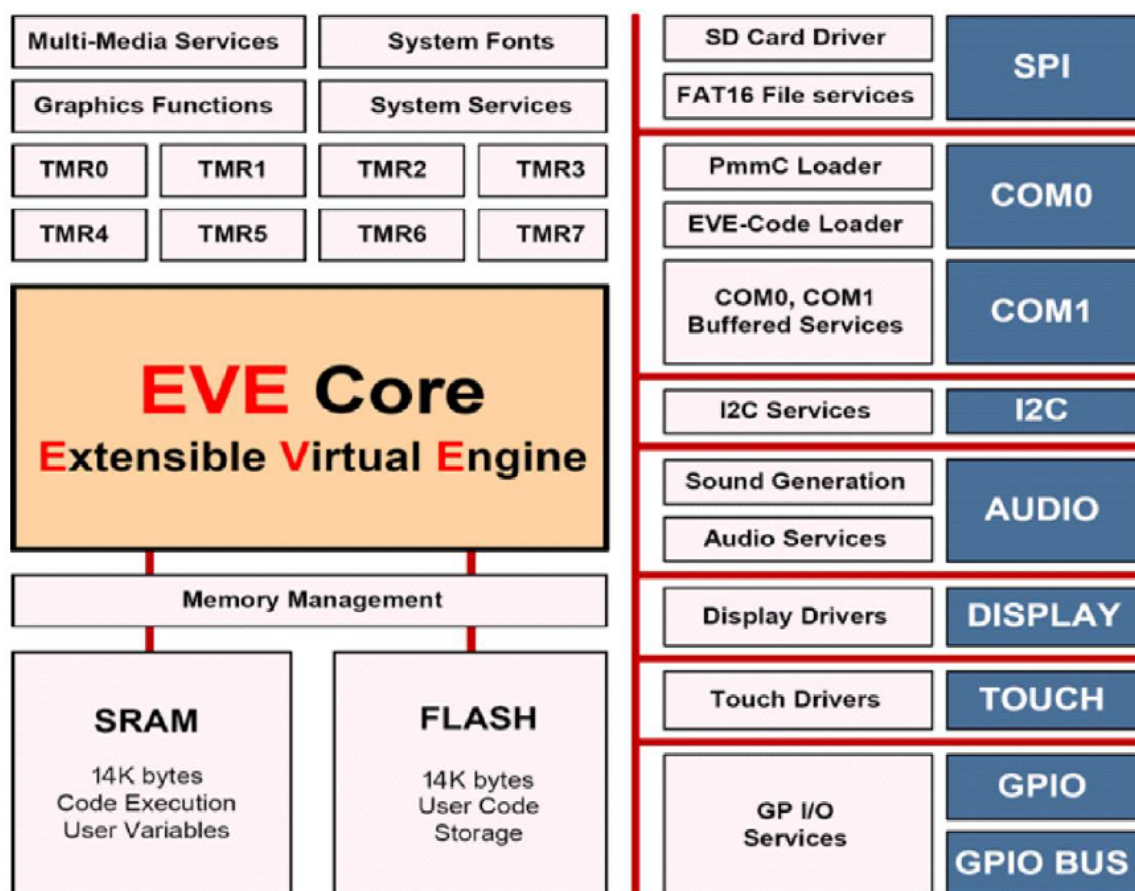
PICASO Internal Block Diagram
