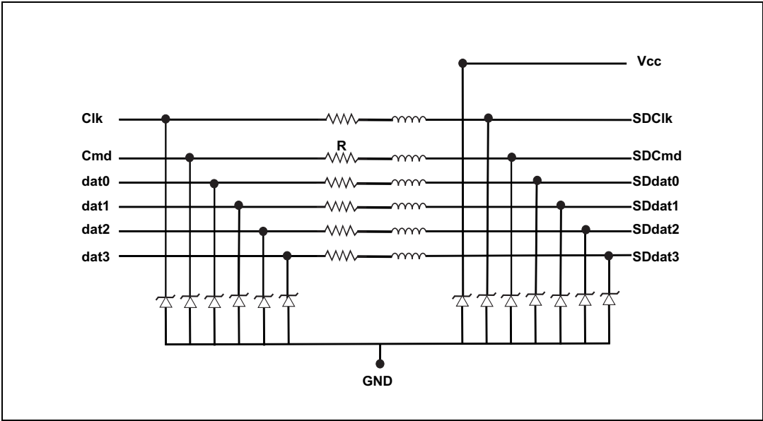
Figure 3. Functional schematic
