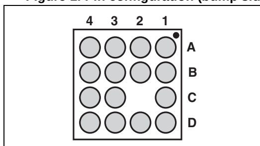
Figure 1. Pin configuration (bump side)
