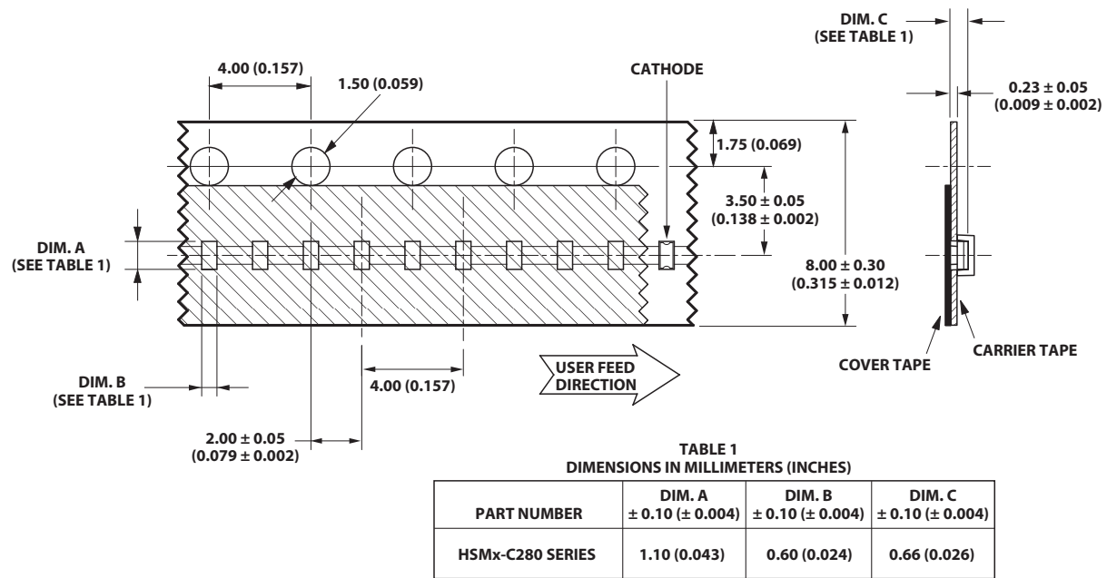
Figure 11. Tape dimensions.
