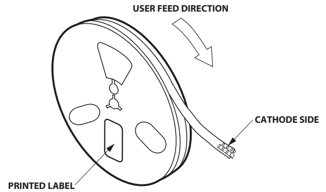
Figure 9. Reeling orientation.
