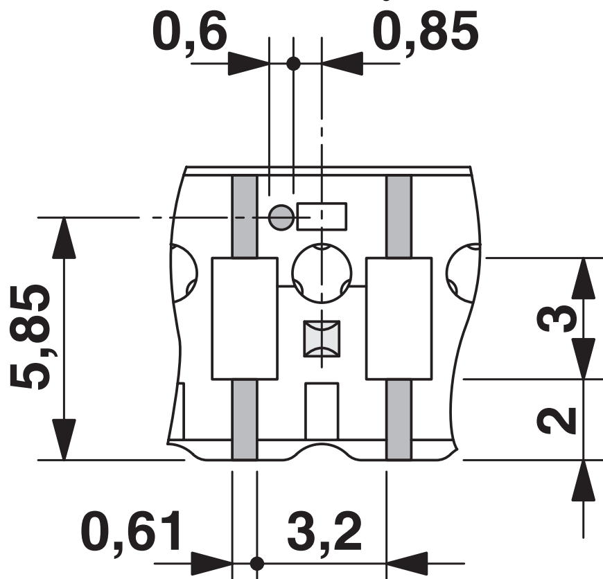
Dimensional drawing
