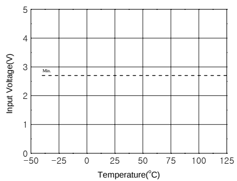
Figure 15b. Logic 1 Input Voltage vs Temperature
