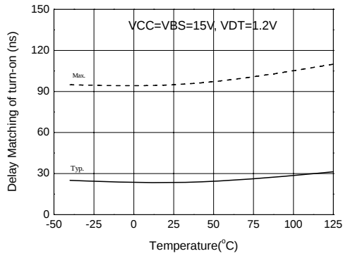
Figure 32. Turn-On Delay Matching vs Temperature
