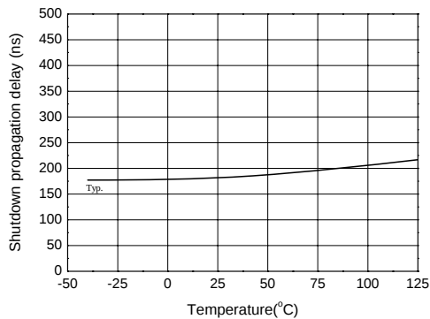
Figure 34. Shutdown Propagation Delay vs Temperature
