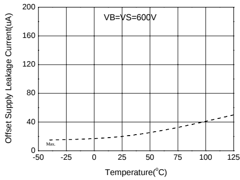
Figure 20a. Offset Supply leakage Current vs Temperature
