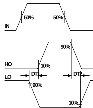
Figure 6. Dead Time Waveform Definitions
