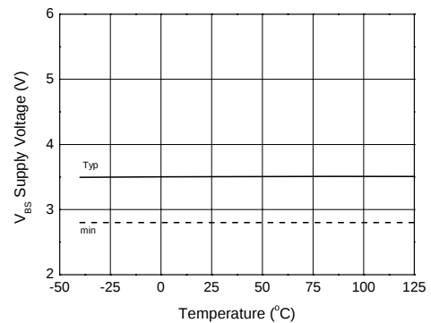
Figure 25b. VBS UnderVoltage Threshold(-) vs Temperature
