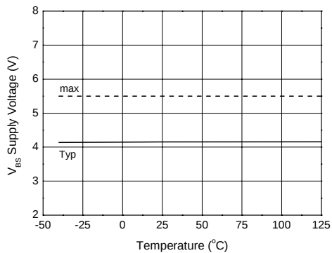
Figure 25a. VBS UnderVoltage Threshold (+) vs Temperature
