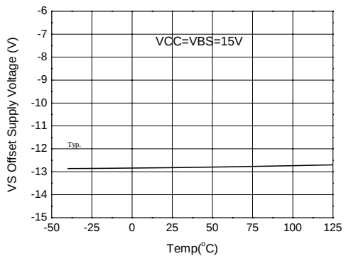
Figure 35. Maximum VS Negative Offset of vs Temperature
