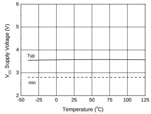
Figure 24b. VCC UnderVoltage Threshold(-) vs Temperature
