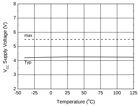
Figure 24a. VCC UnderVoltage Threshold (+) vs Temperature
