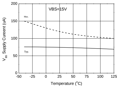
Figure 21. VBS Supply Current vs Temperature
