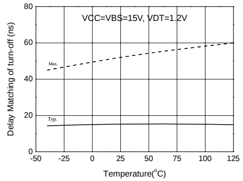
Figure 33. Turn_Off Delay Matching vs Temperature
