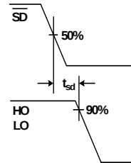
Figure 4. Shutdown Waveform Definitions
