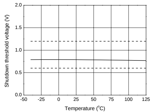
Figure 29. Shutdown Threshold of vs Temperature
