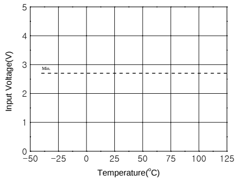
Figure 15a. Logic 0 Input Voltage vs Temperature
