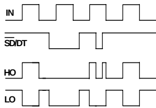
Figure 1. Input/output Timing Diagram
