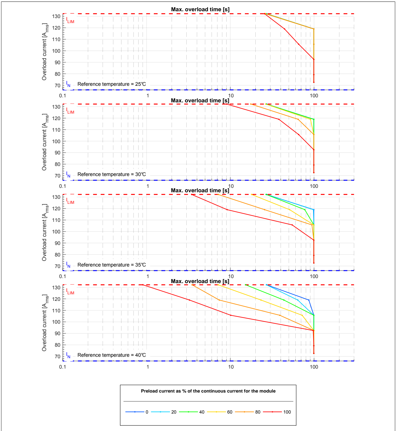
Figure 1: 8BVI0660HWSx.0x8-1 - Overload characteristics, overload response - WARNING
