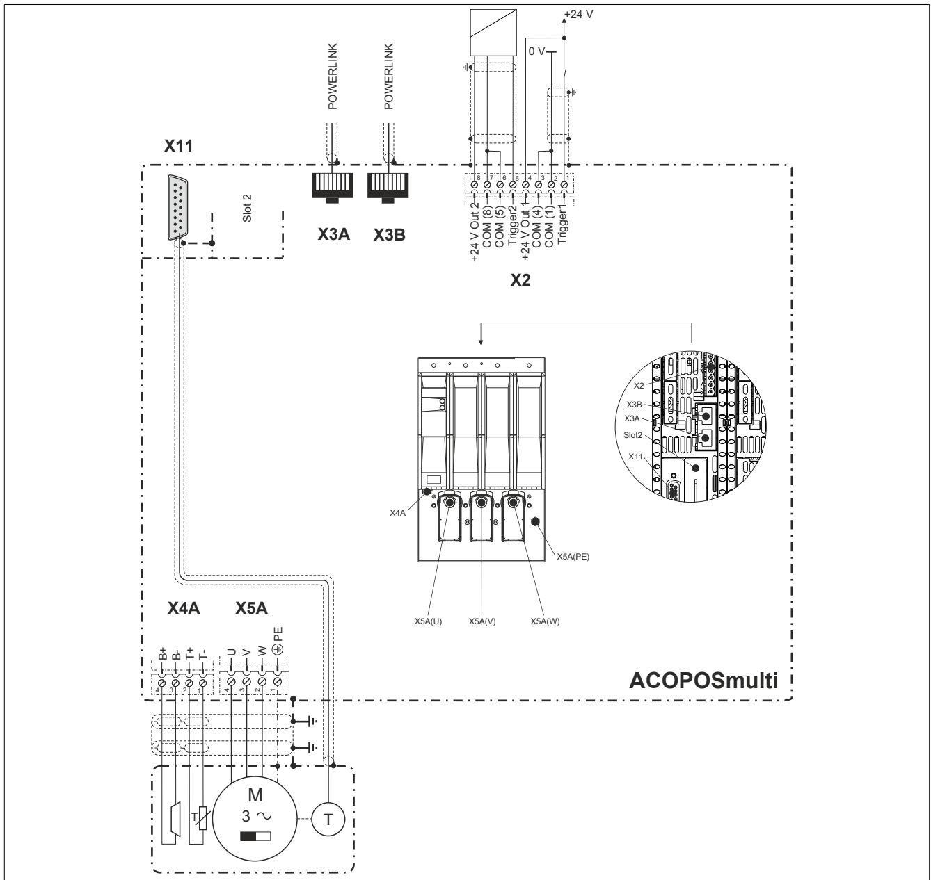
Figure 4: Pinout overview
