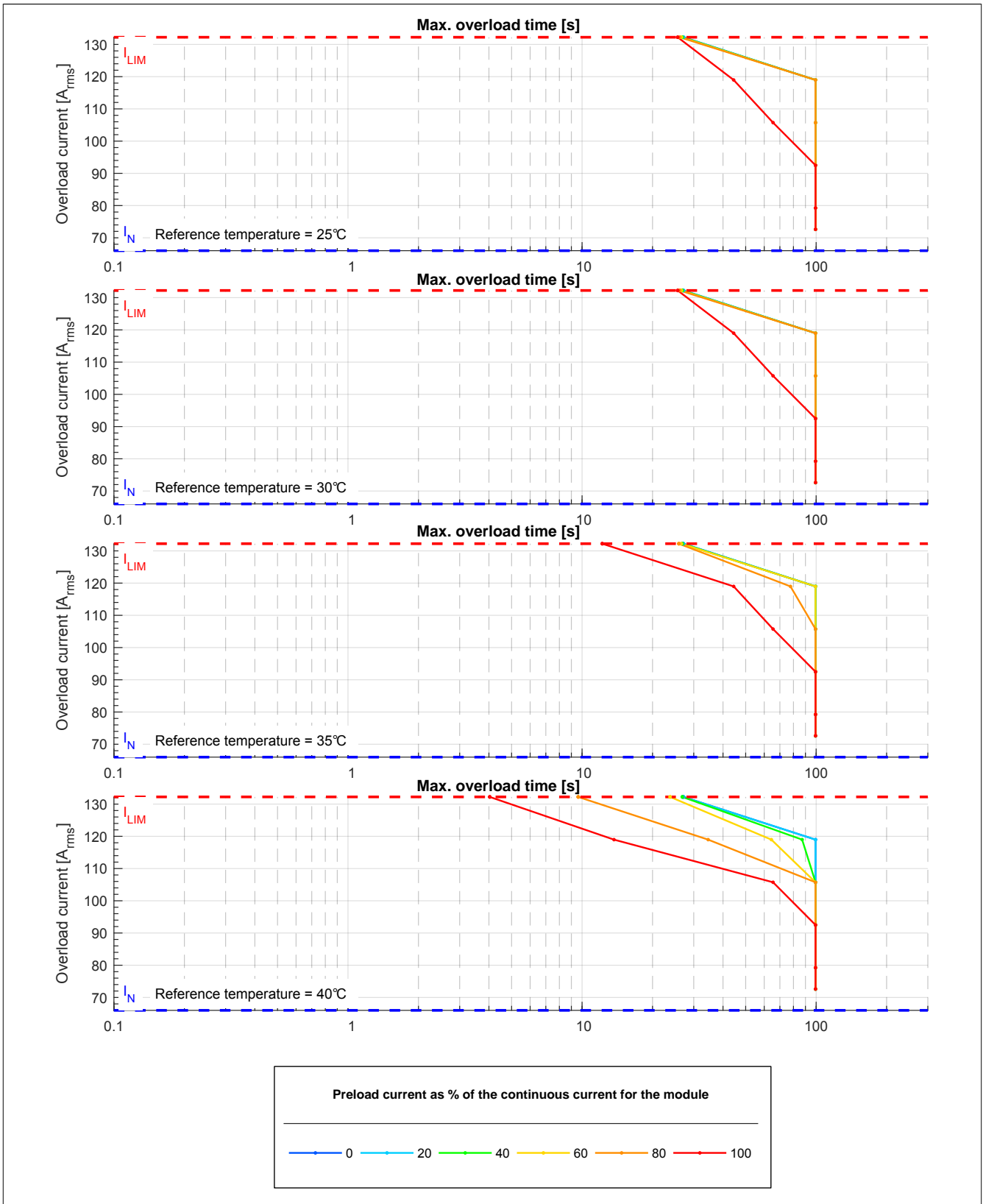
Figure 2: 8BVI0660HWSx.0x8-1 - Overload characteristics, overload response - ERROR+STOP
