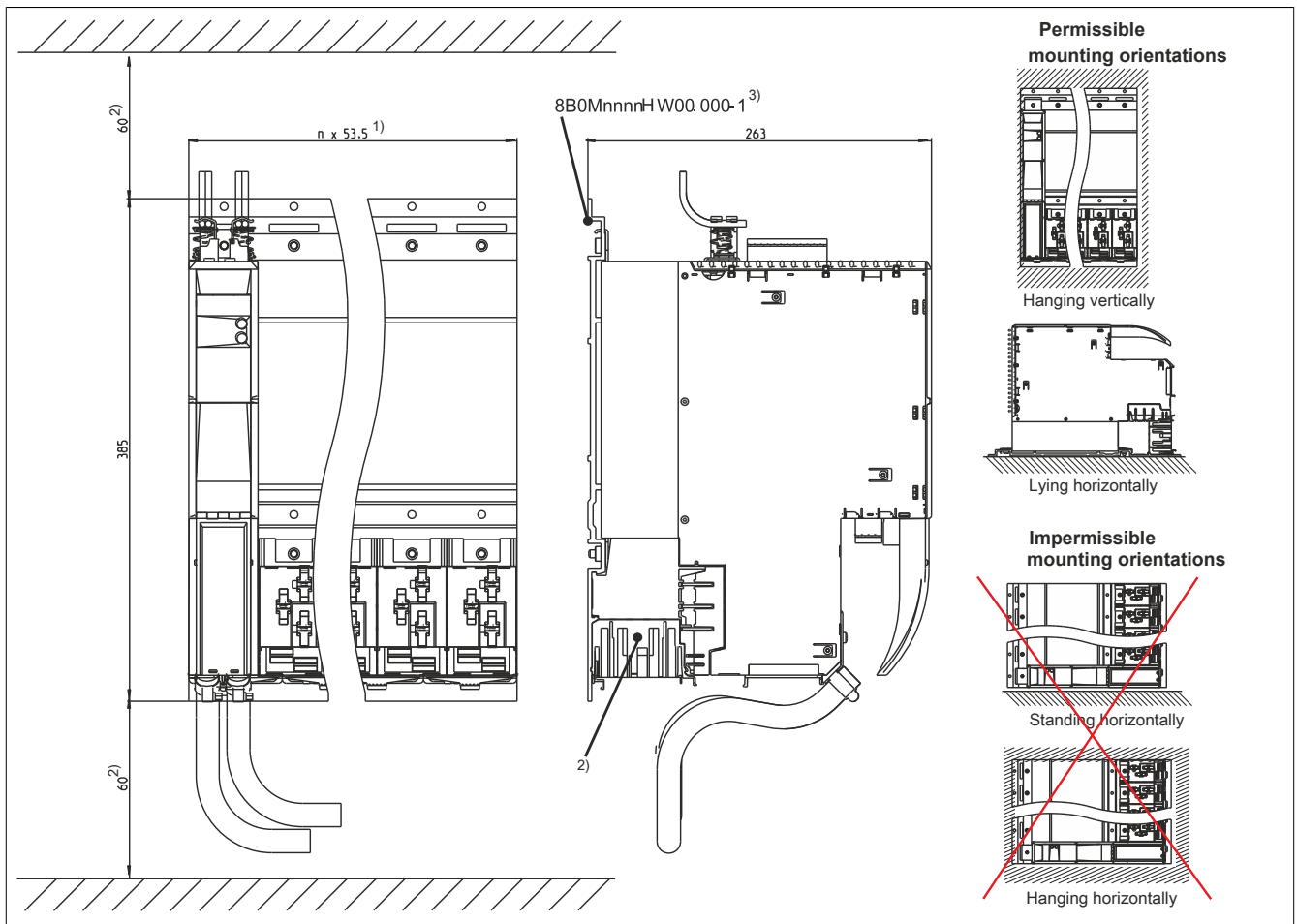
Figure 3: Dimension diagram and installation dimensions
