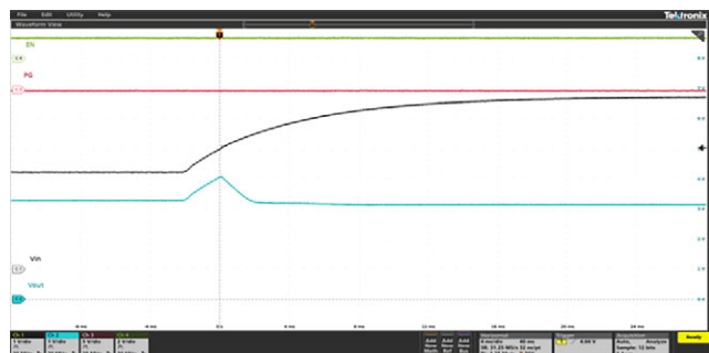
Fig. 25 - Overvoltage Clamp Response - SiP32436 ROVSEL = GND, C_{OUT} = 220 \mu F , I_{OUT} = 200 \text{ mA} , V_{IN} ramped up from 3.3 V to 5.8 V
