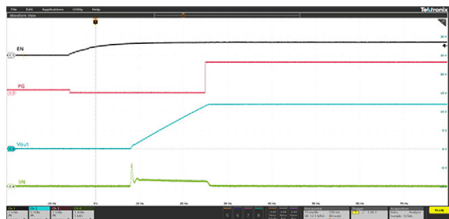
Fig. 50 - Power Start-Up With V IN Ramp
