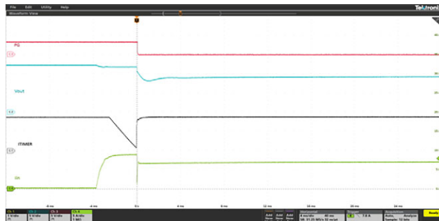
Fig. 28 - Active Current Limit Response - SiP32436 V_{IN} = 12 \text{ V} , CITIMER = 3.3 nF, C_{OUT} = 220 \mu F , R_{ILM} = 680 \Omega , Resistor stepped from Open \Omega \rightarrow 1.3 \Omega
