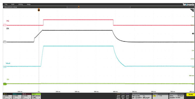
Fig. 19 - Power Up and Down With EN/UVLO Control V_{IN} = 12\text{ V} , C_{OUT} = 22\text{ }\mu\text{F} , C_{SS} = 3.3\text{ nF} , V_{EN}/UVLO ramped from 0\text{ V} \rightarrow 1.4\text{ V} \rightarrow 0\text{ V}
