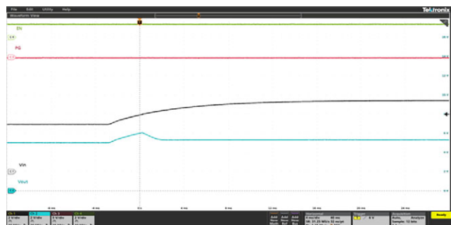
Fig. 26 - Overvoltage Clamp Response - SiP32436 ROVSEL = Open, C_{OUT} = 220 \mu F , I_{OUT} = 200 \text{ mA} , V_{IN} ramped up from 5 V to 7.5 V
