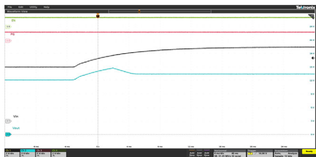
Fig. 27 - Overvoltage Clamp Response - SiP32436 ROVSEL = 390 k \Omega , C_{OUT} = 220 \mu F , I_{OUT} = 200 \text{ mA} , V_{IN} ramped up from 12 V to 16.5 V
