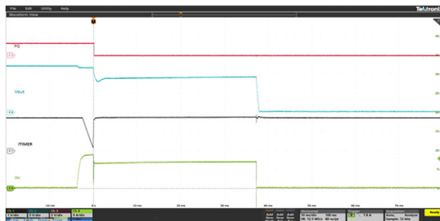
Fig. 29 - Active Current Limit Response Followed by TSD - SiP32436 V_{IN} = 12 \text{ V} , CITIMER = 3.3 nF, C_{OUT} = 220 \mu F , R_{ILM} = 680 \Omega , Resistor stepped from Open \Omega \rightarrow 1.3 \Omega
