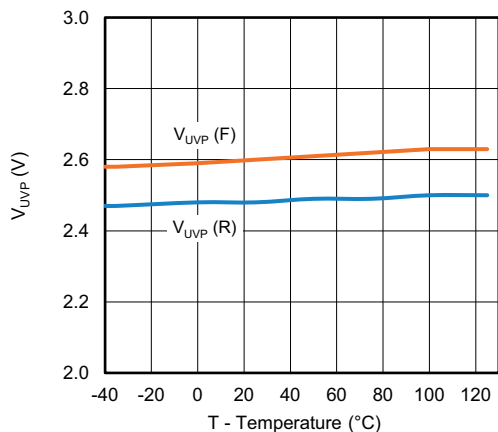
Fig. 3 - V_{\text{IN}} UVLO vs. Temperature
