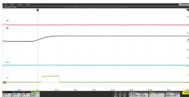
Fig. 34 - Power Up into Short-Circuit V_{IN} = 12\text{ V} , C_{OUT} = \text{Open} , I_{OUT} short-circuit to GND, R_{ILM} = 680\text{ }\Omega , V_{EN}/V_{LO} stepped from 0\text{ V} \rightarrow 3.3\text{ V}
