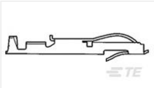
TE Part #583649-3 CONT.CRP.SNAP TW.LF.STRIP
