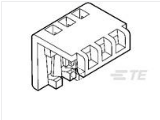
TE Part #643075-4 04P MTA100 MOLDED COVER
