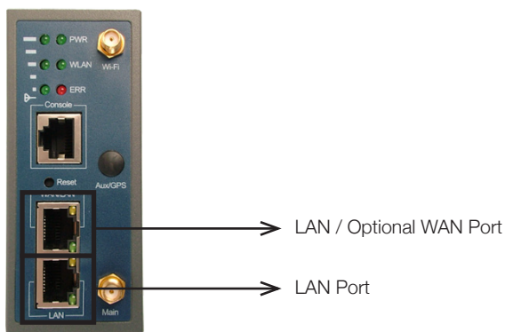
Figure 15. QUARTZ LAN / WAN Connection
