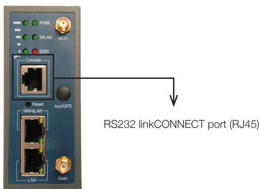
Figure 11. RS232 serial port
