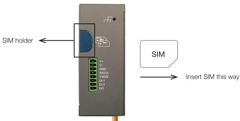
Figure 17. SIM holder
