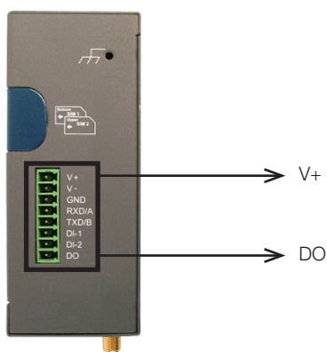
Figure 16. Input/Output
