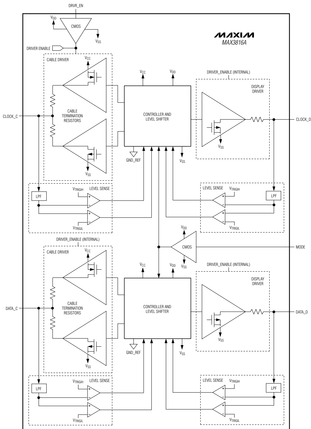
Figure 2. Functional Diagram
