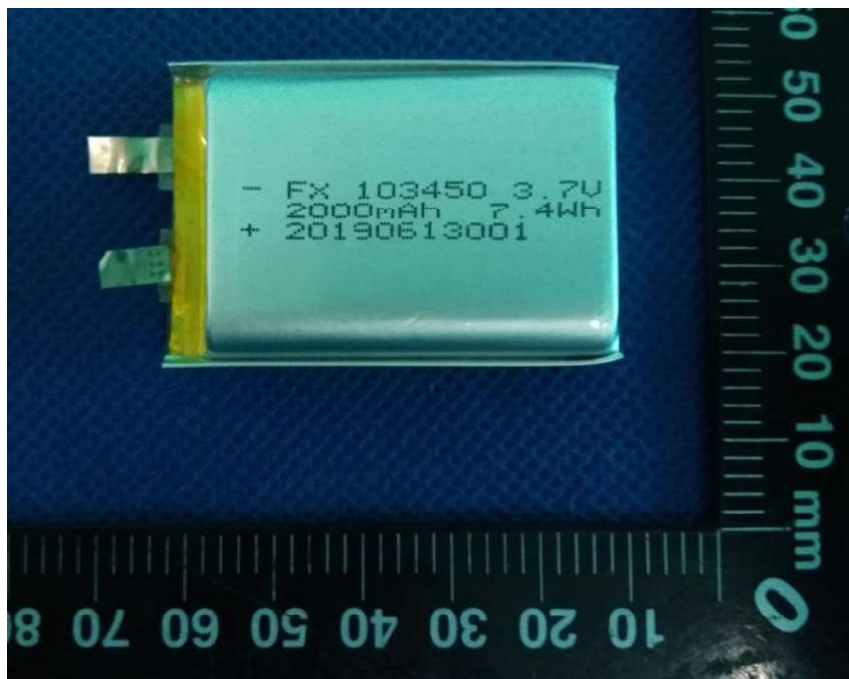
元件电池 View of the component cell
