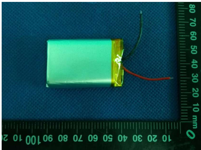
电池组外观 2 View of the battery 2
