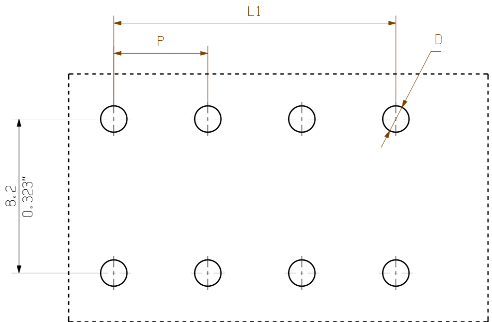
Hole pattern
