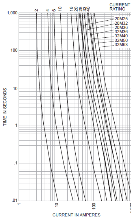
Time-Current Characteristic Curve (Full Size Curves Available)
