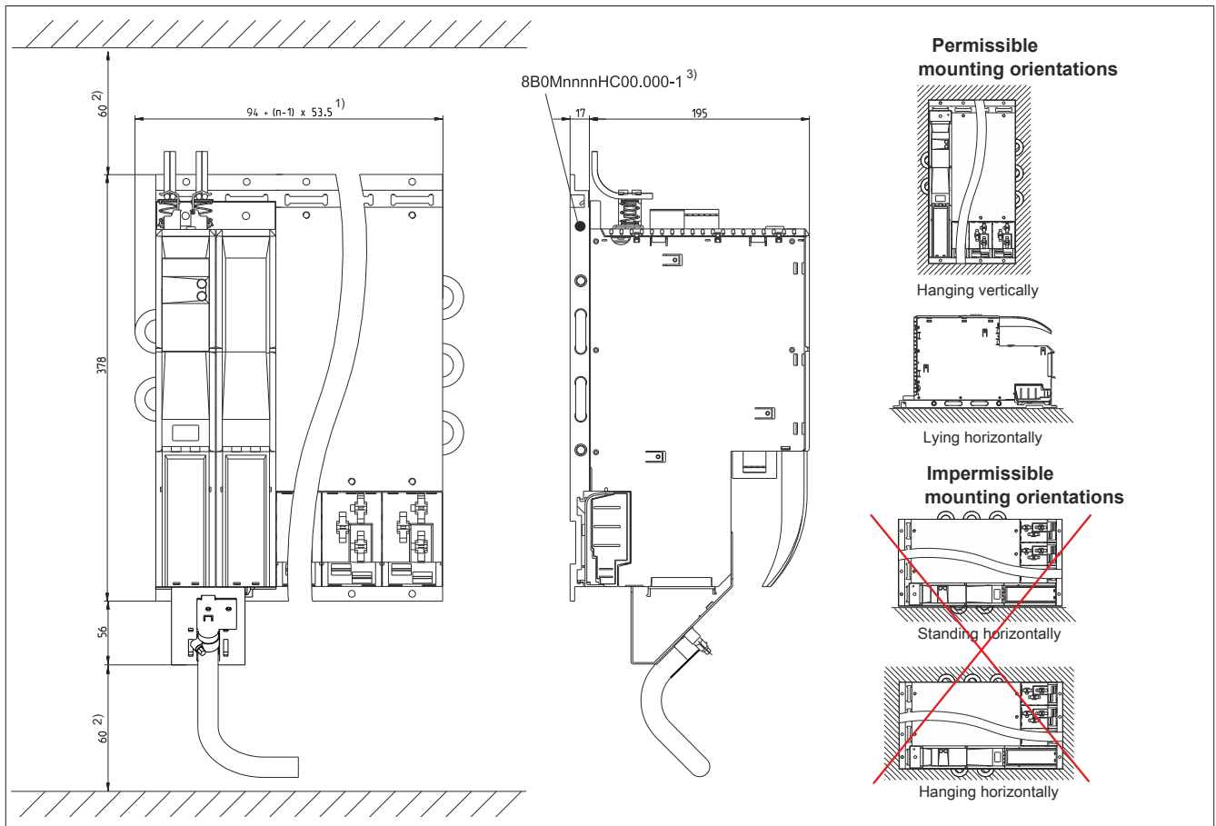
Figure 6: Cold plate - Dimension diagram and installation dimensions
