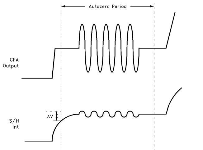
Figure 8. Lowpass Filter Delays Input to Sample and Hold
