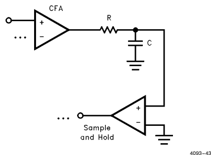
Figure 7. Caution: Lowpass Filter Does Not Work in NTSC Applications
