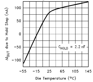
Hold Step ( \Delta I_{OUT} ) vs Temperature
