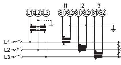
Fig. 10 Three-phase system with neutral (4-wire), balanced load, 1 CT and 1 VT/PT
