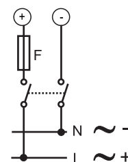
Fig. 19 Auxiliary power supply. 250 V [T] 630 mA fuse (F).
