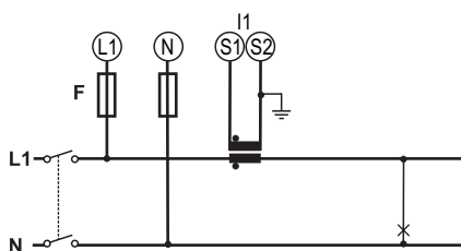
Fig. 17 Single-phase system (2-wire), 1 CT, 315 mA fuse (F).
