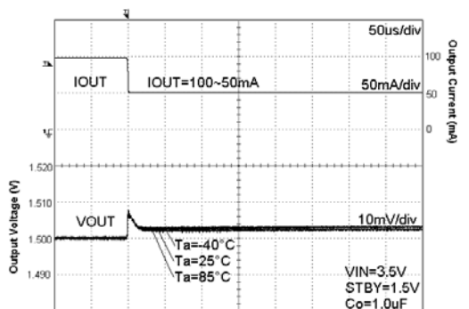
Fig. 23 Load Response
