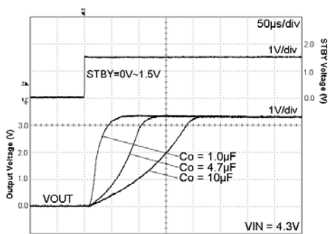
Fig. 173 Start Up Time I_{out} = 0\text{mA}
