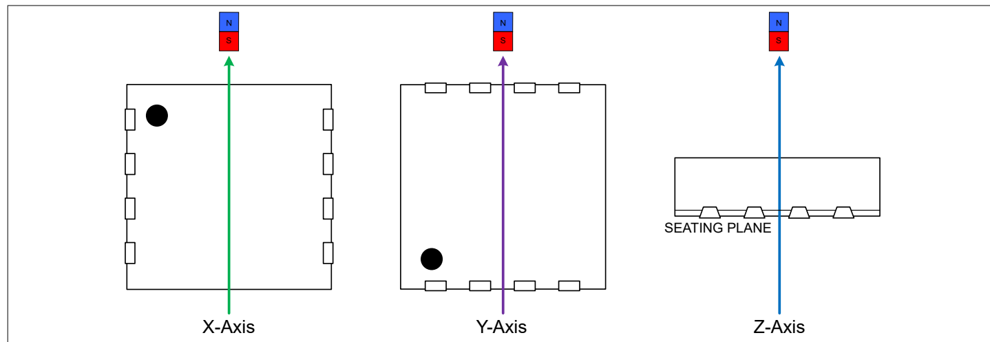
Figure 3 Definition of magnetic field direction
