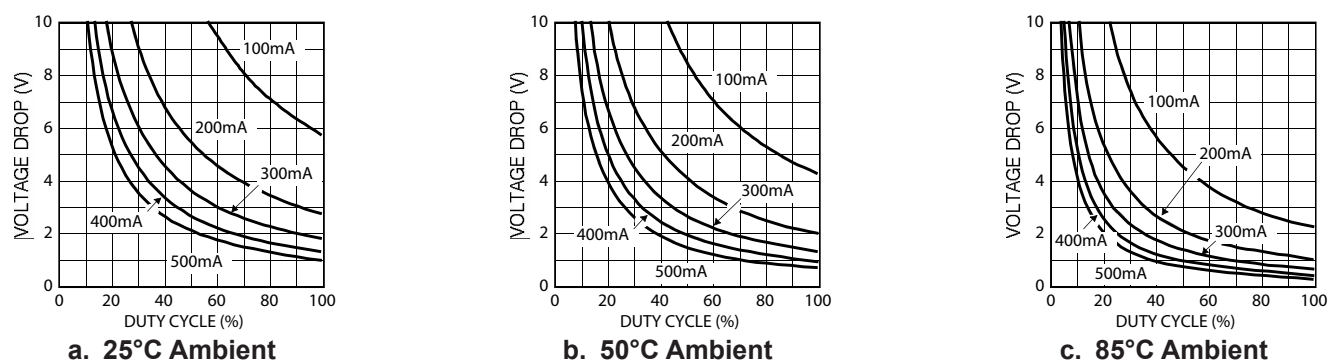
Figure 2. MIC5219-x.xBM5 (SOT-23-5) on 1-inch² Copper Cladding
