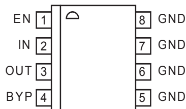
MIC5219YMM MIC5219BMM MM8™ MSOP-8 Adjustable Voltage
