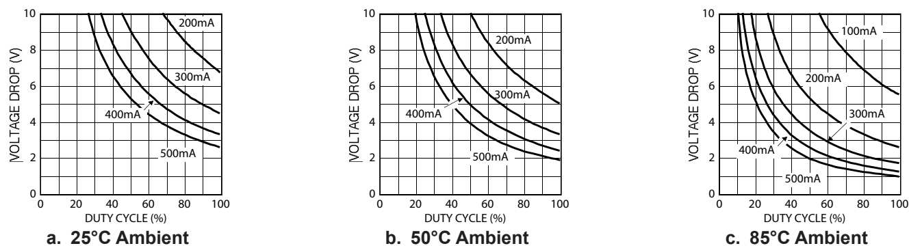
Figure 4. MIC5219-x.xBMM (MSOP-8) on 1-inch² Copper Cladding
