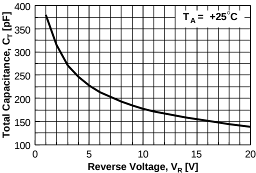
Figure 3. Total Capacitance
