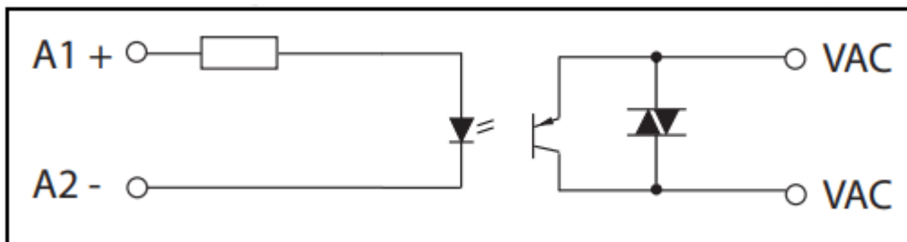
Simplified circuit diagram 2 A, 240 VAC version with Triac Output
