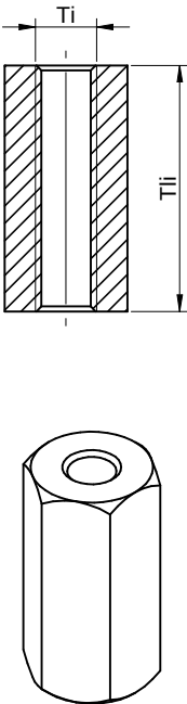
sectional drawing A-A
