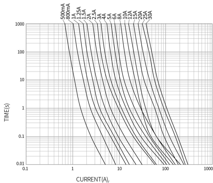
HC10SR AVERAGE I-T CHARACTERISTICS CURVE (FOR REFERENCE ONLY)
