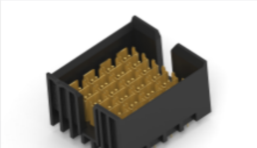
TE Part #2274854-1 SW HDR ASM, 4P, 6C, 85O, PIC
