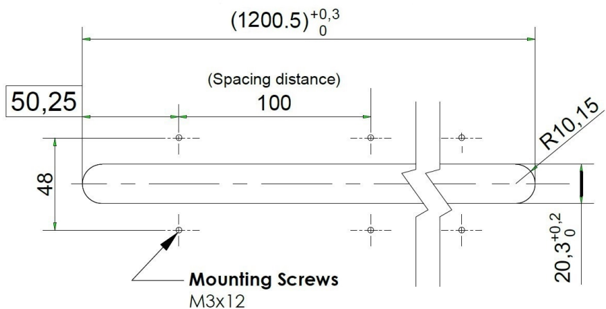
Mounting Diagram_Clip
