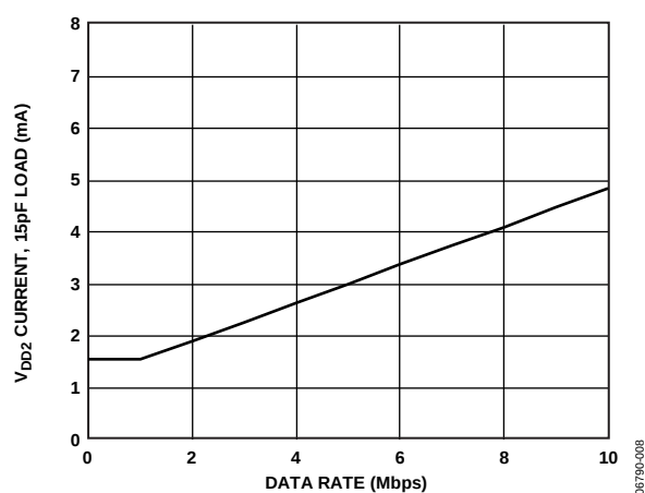
Figure 8. Typical Total V_{DD2} Supply Current vs. Data Rate (15 pF Output Load)
