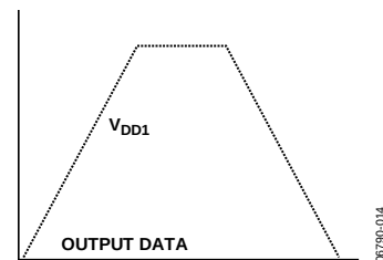
Figure 14. V_{DD1} Power-Up/Power-Down Characteristics, Input Data = Low
