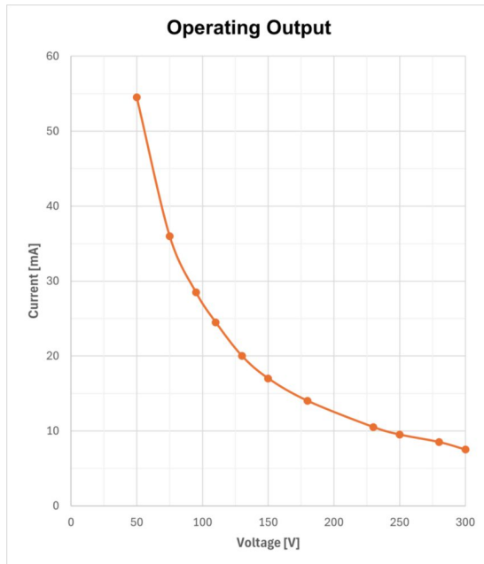
Operating Output LUX365 MIDI 300V 3W LiFePO4 3H
