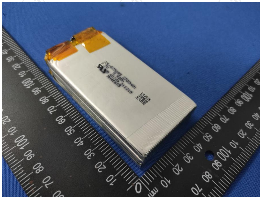
Picture 5. Cell view
