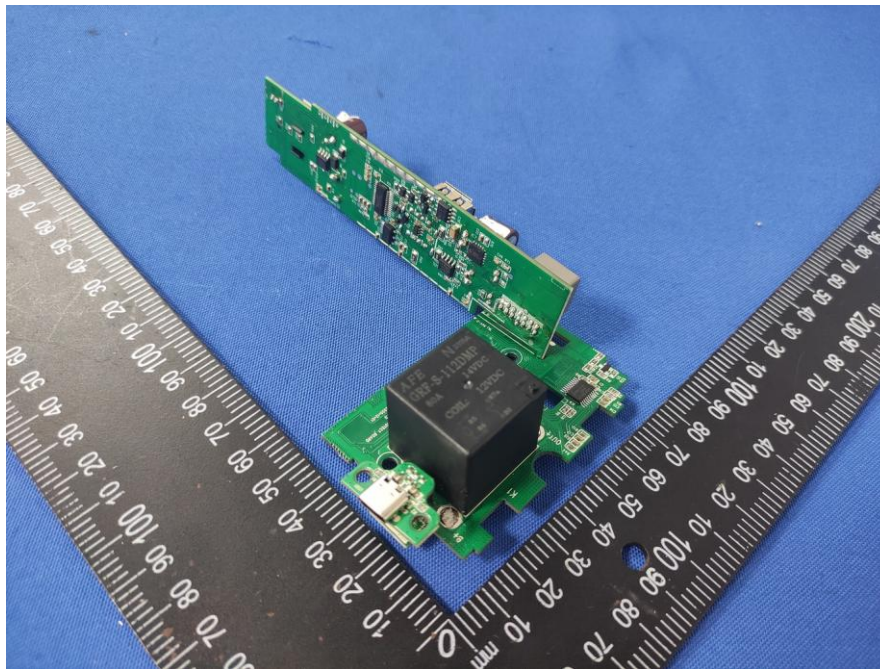
Picture 7. Protection board view
