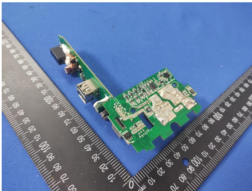
Picture 8. Protection board view
