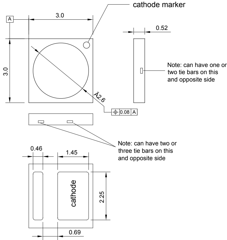
Figure 13: Mechanical dimensions for LUXEON 3030 2D.
