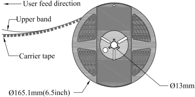
Figure 17: Reel dimensions for LUXEON 3030 2D.
