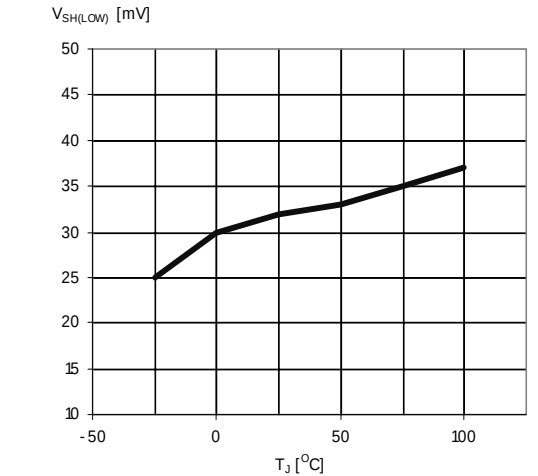
Figure 6. Max. share bus voltage at no load
