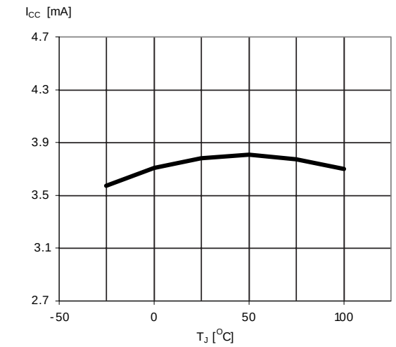
Figure 3. Supply current
