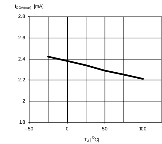
Figure 4. Max CGA current
