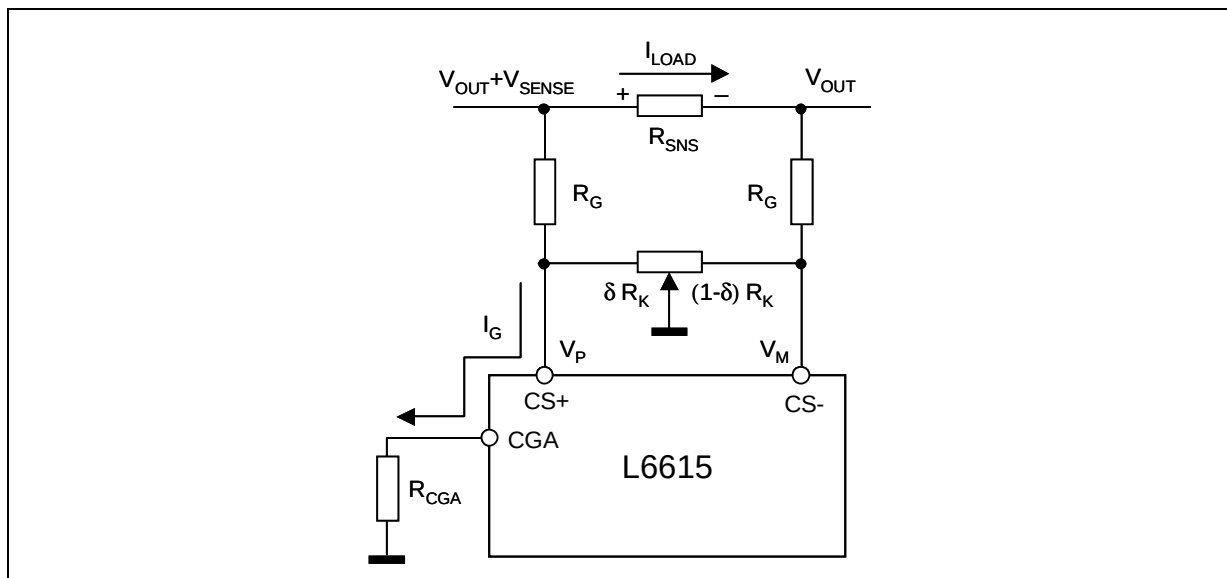
Figure 16. Offset Trimming
