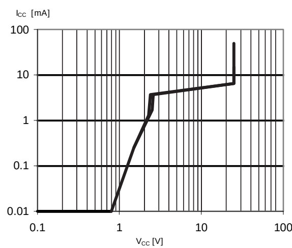
Figure 3. Supply current
