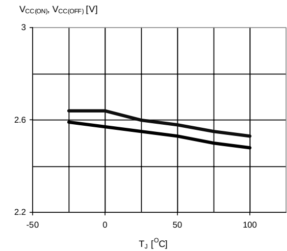
Figure 1. Turn-on and turn-off voltage
