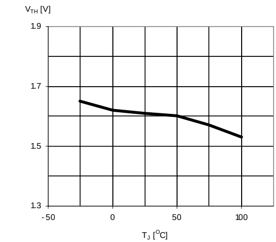
Figure 5. High side/low side sensing switchover threshold
