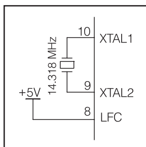
Fig. 4 - Crystal Oscillator
